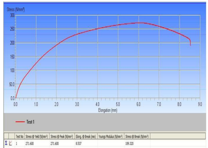
Figure 9. Tensile test diagram for specimen quenched in distill water
