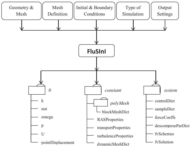
Figure 2: FLUSINI general setup flow chart.
