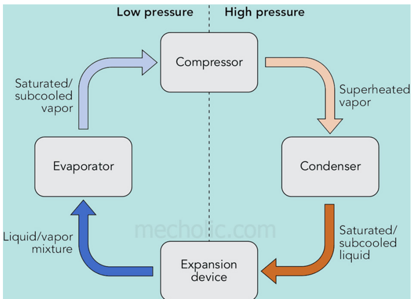
Figure 1: VCR system [10].
