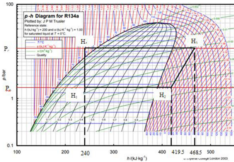
Figure 6: R134a-ZnO p-h chart.
