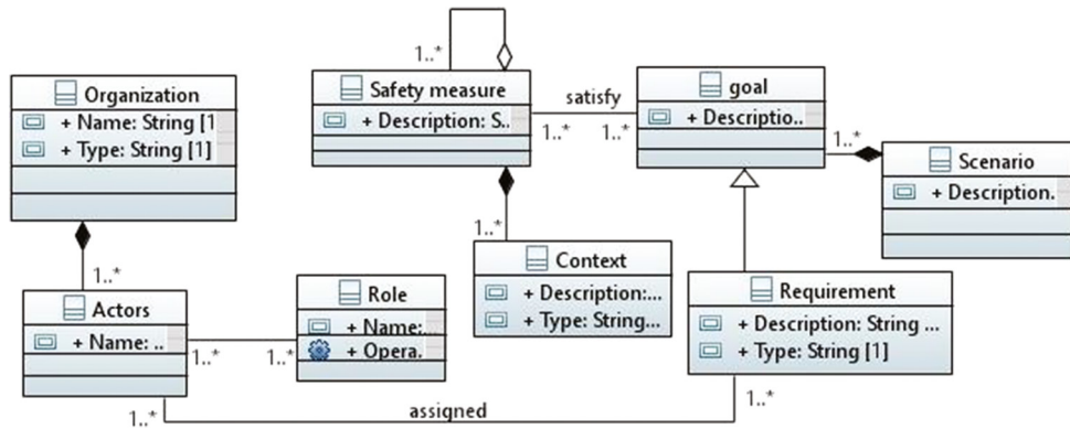
Figure 4: UML class diagram of safety rule-related concepts.
