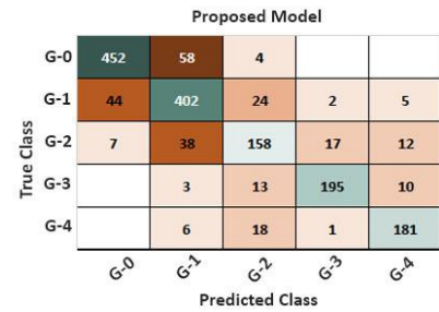
Figure 7. The confusion matrix of proposed model ((DenseNet201+DarkNet53+ShuffleNet)+NCA+SVM)
