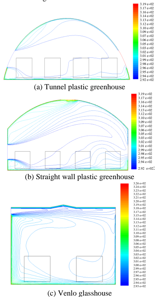
Figure 9. Computed contours of air temperature ( \text{K} ) at the middle of the greenhouses
