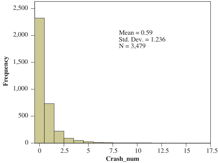
Figure 1: Distribution of hourly crashes.
