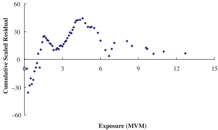
Figure 3: Cumulative scaled residual versus EXPO.
