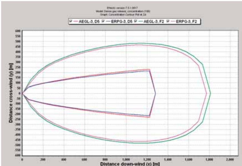
Figure 3: Concentration contour plots for F_2 corresponding to AEGL-3 and ERPG-3; D5 and F2 atmospheric stability classes.
