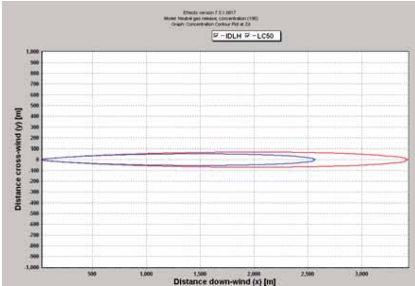
Figure 1: Concentration contour plots for CO corresponding to IDLH and LC50; F2 atmospheric stability class.
