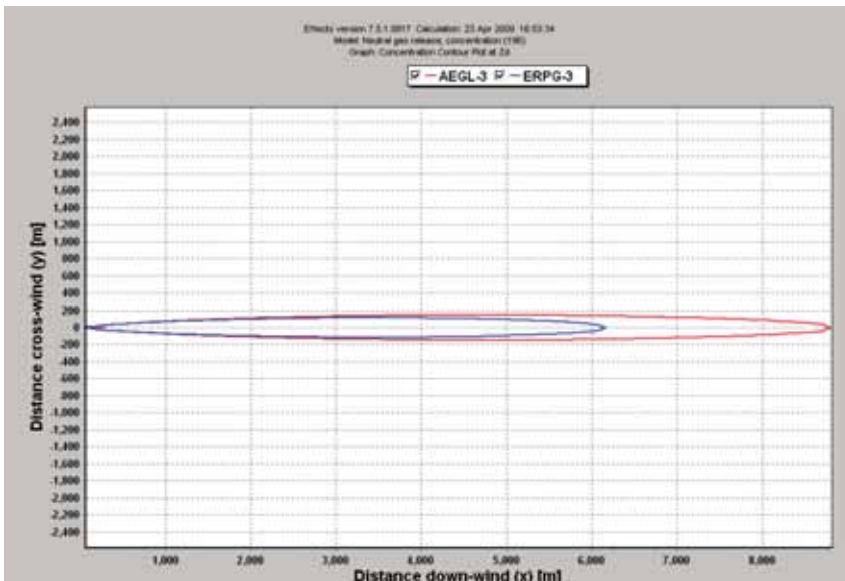
Figure 2: Concentration contour plots for CO corresponding to AEGL-3 and RPG-3; F2 atmospheric stability class.
