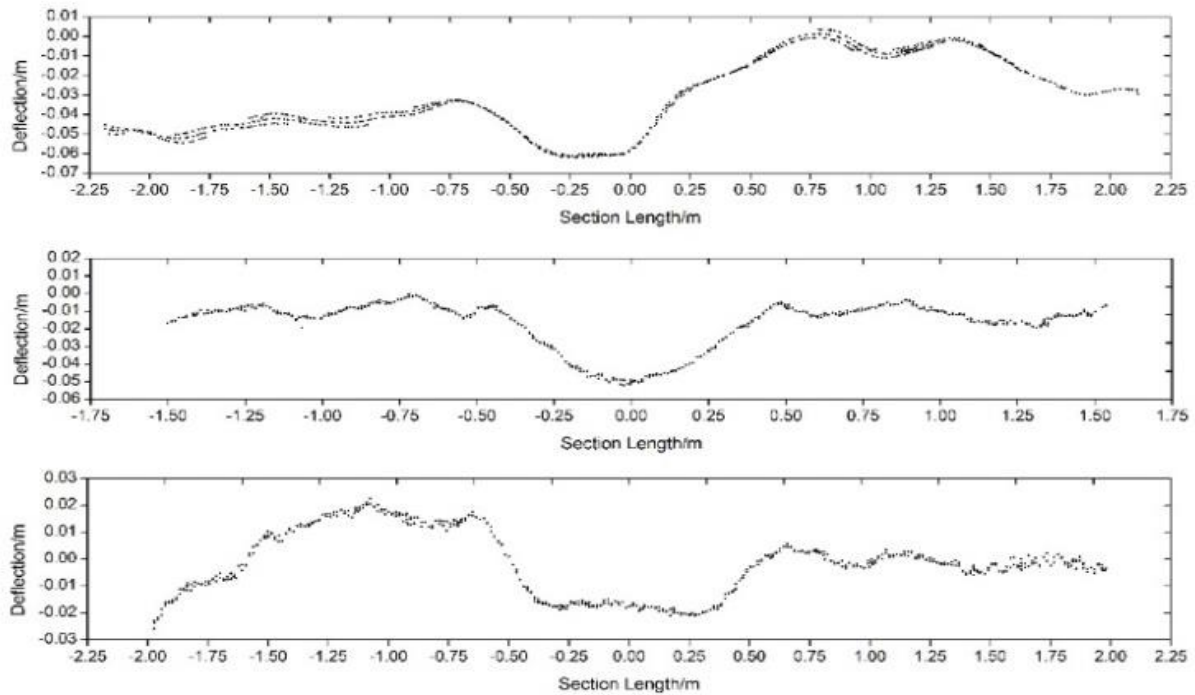
Fig.8. The Distribution of Point Cloud in Sections 1-3
