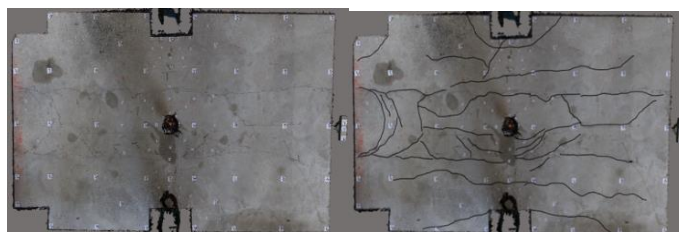
Fig.14. Distribution of Cracks on the Surface of the Box Girder after Loading
