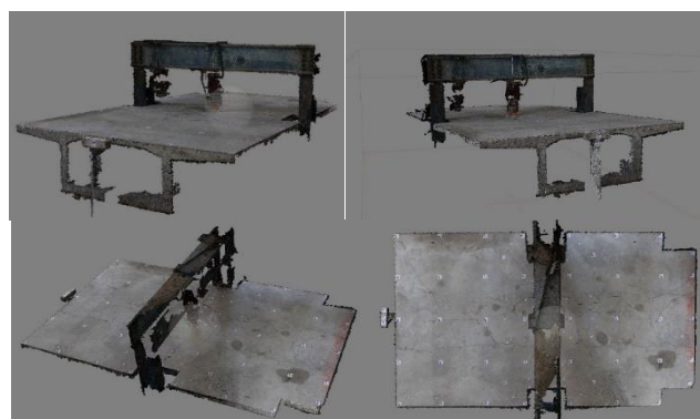
Fig.2. Three Dimensional Point Cloud Reconstruction Effect of Box Girder Specimen
