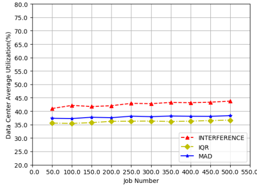
Fig.3. Average CPU Utilization of Datacenter at Different Numbers of Servers and VMs
