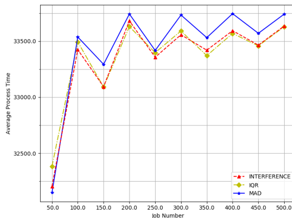
Fig.6. Average process time of VMs at different numbers of servers and VMs
