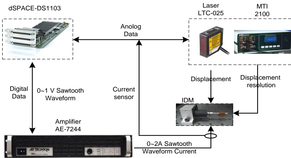
Fig.6. The framework of experimental system
