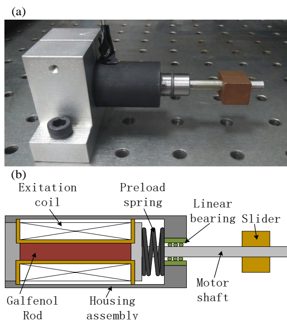
Fig.2. The Magnetostrictive IDM (a) Photo of the motor (b) Schematic of the motor
