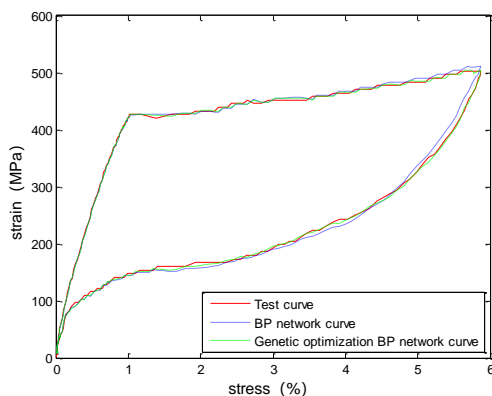
(a) Stress-strain curve comparison
