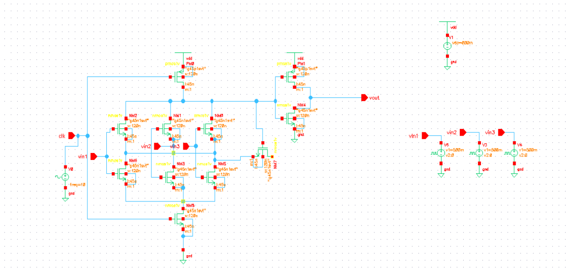
Fig.9. Noise immune Dynamic circuit
