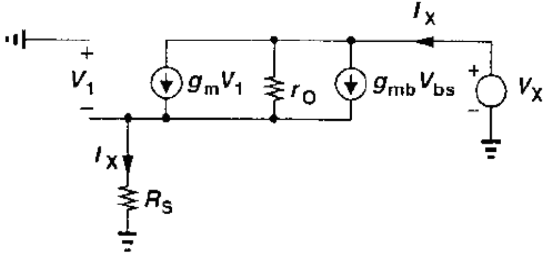
Fig.4. Large signal analysis
