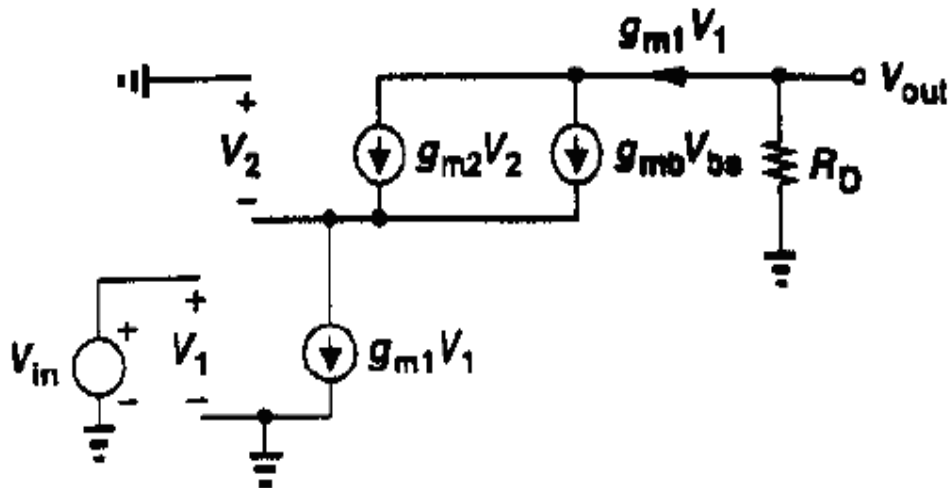
Fig.5. Small signal equivalent circuit of cascode circuit
