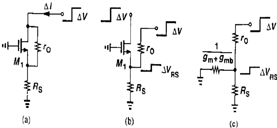
Fig.7. Equivalent circuits
