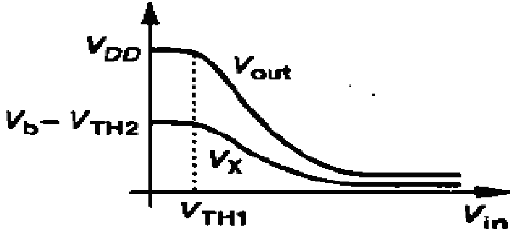
Fig.3. Input output characteristics of a cascode stage
