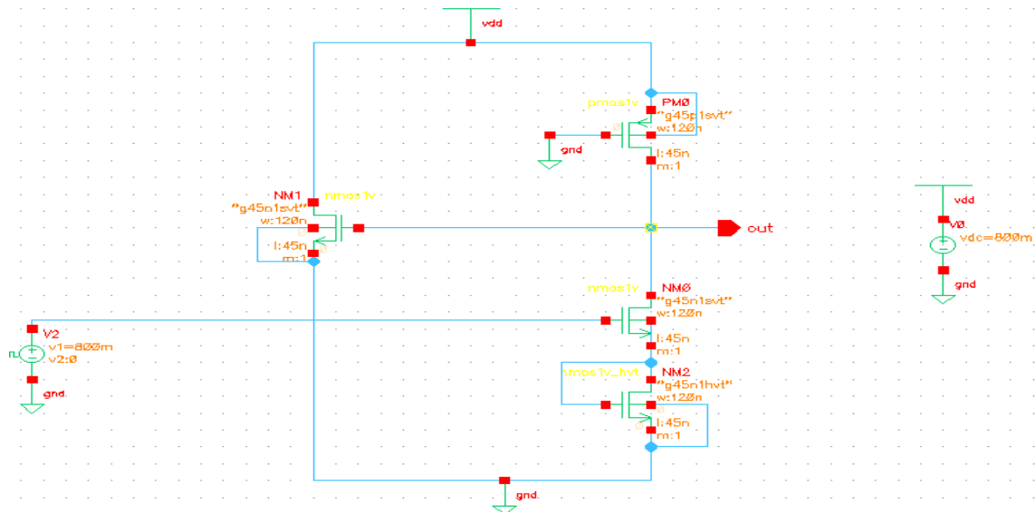
Fig.8. Proposed Highly Stable Current Balanced Logic (HCBL)
