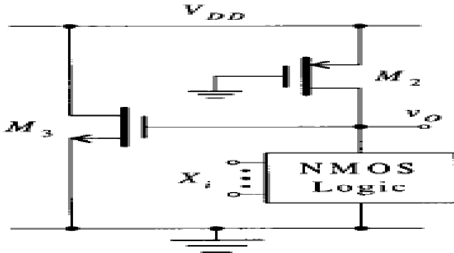
Fig.1. Current Balanced Logic family
