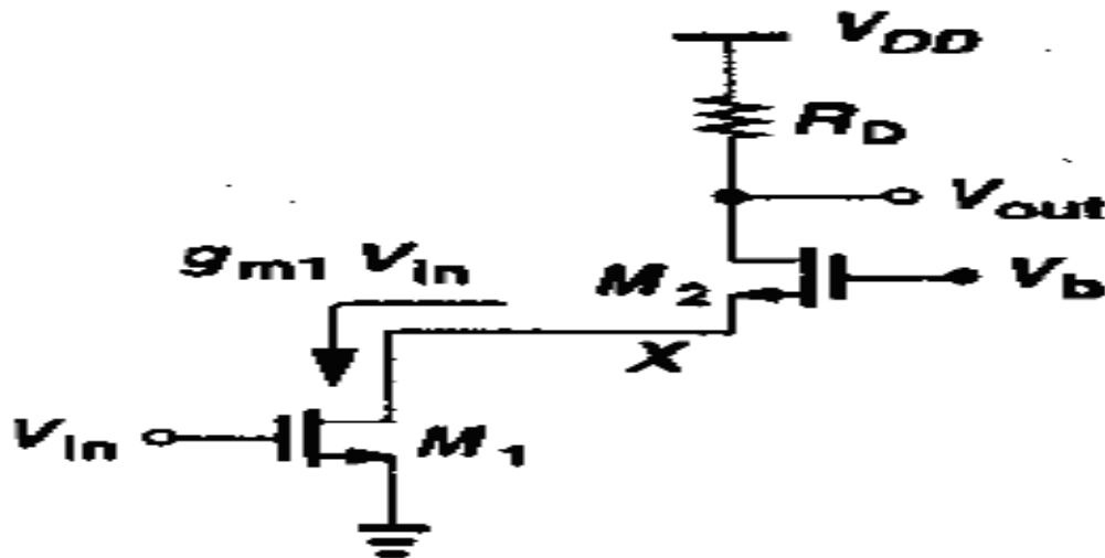
Fig.2. Gain improvement circuit
