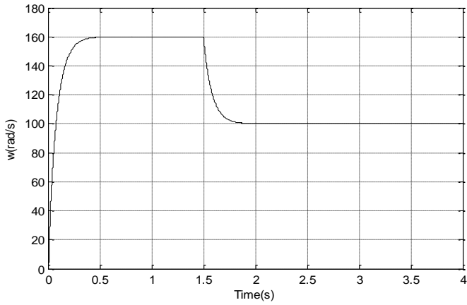
figure 4.a: Speed response
