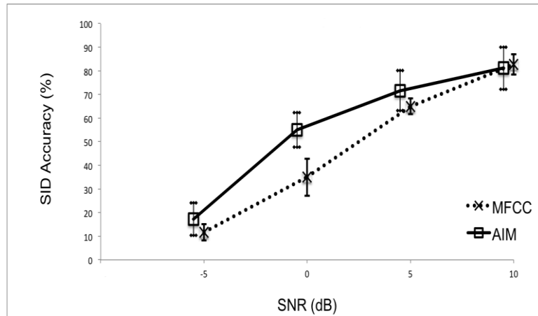
Fig.9. Speaker Identification (SID) Accuracy (%) of the SAI-based and MFCC-based Systems for the Corpus of 180 Speakers Using Multi-talker Babble Noise. The Error Bars Represent the Standard Error of the Mean (Among the Levels of SID Accuracy of the 3 Subsets of 60 Speakers)
