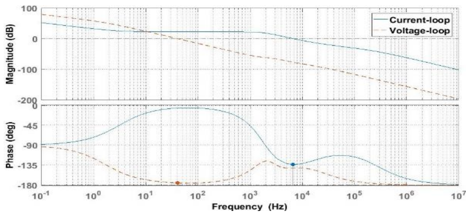
Fig.9. Bode Plot of the Dual-loop Compensated in the DCM
