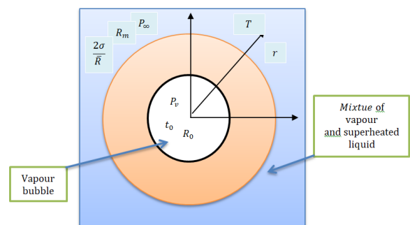
Figure 1. Sketch of bubble dynamic.
