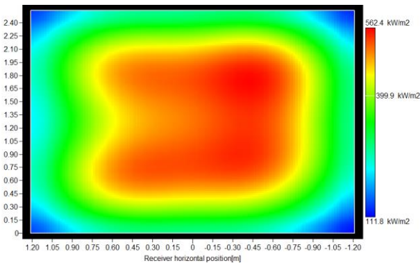
Figure 24. Incident flux on the receiver for SM 1.2 and heliostat type 1
