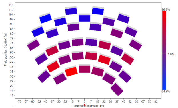
Figure 21. Solar field SM 1.3 Type 1 heliostats
