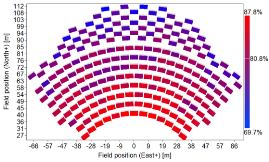
Figure 2. Solar field SM 1.1 Type 3 heliostats
