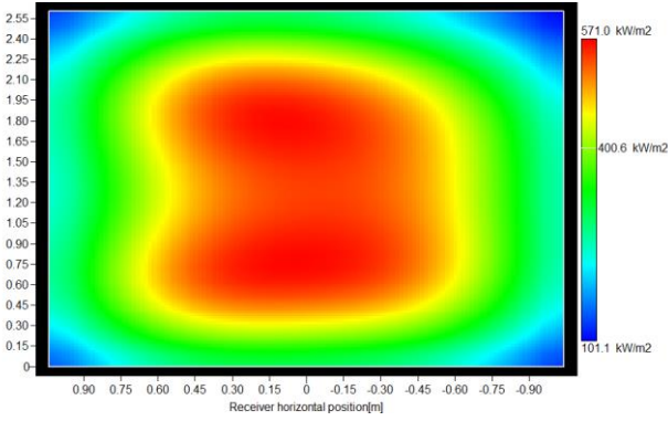
Figure 22. Incident flux on the receiver for SM 1 and heliostat type 1
