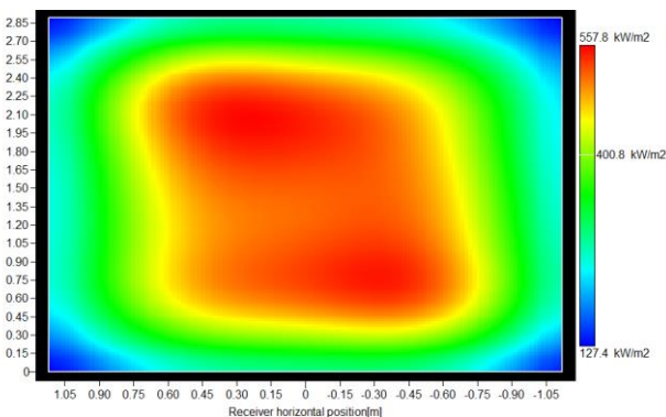
Figure 25. Incident flux on the receiver for SM 1.3 and heliostat type 1
