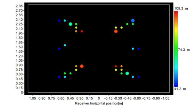
Figure 9. An aiming point of the heliostats chosen for the simulations
