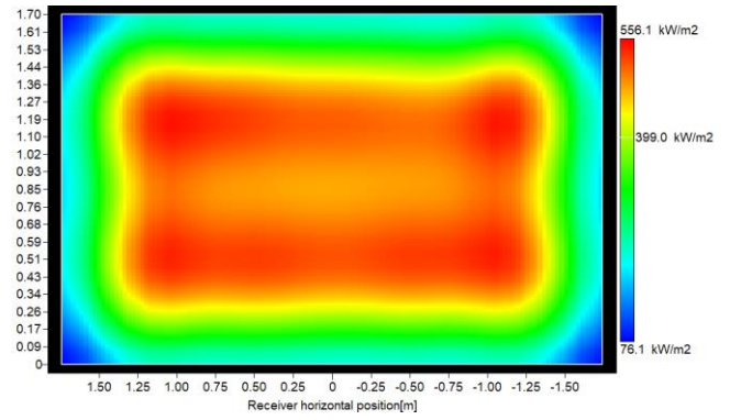
Figure 6. Incident flux on the receiver for SM 1.1 and heliostat type 3
