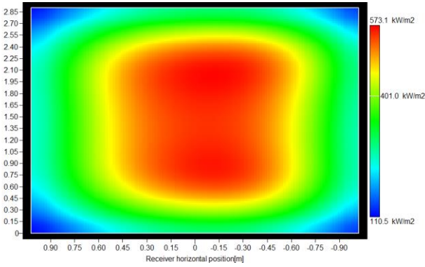
Figure 23. Incident flux on the receiver for SM 1.1 and heliostat type 1
