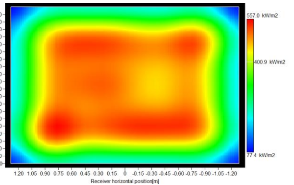
Figure 14. Incident flux on the receiver for SM 1 and heliostat type 2
