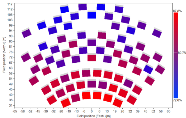
Figure 10. Solar field SM 1 Type 2 heliostats
