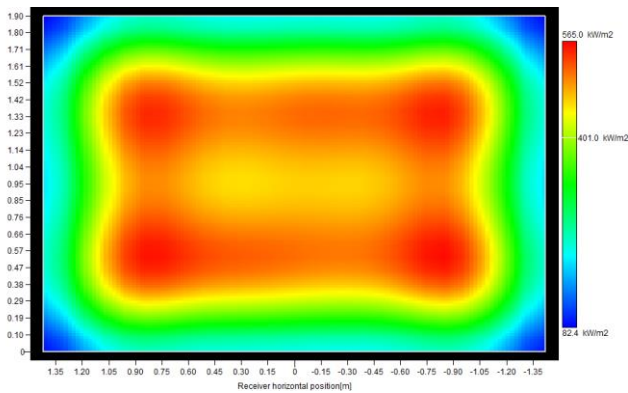
Figure 5. Incident flux on the receiver for SM 1 and heliostat type 3
