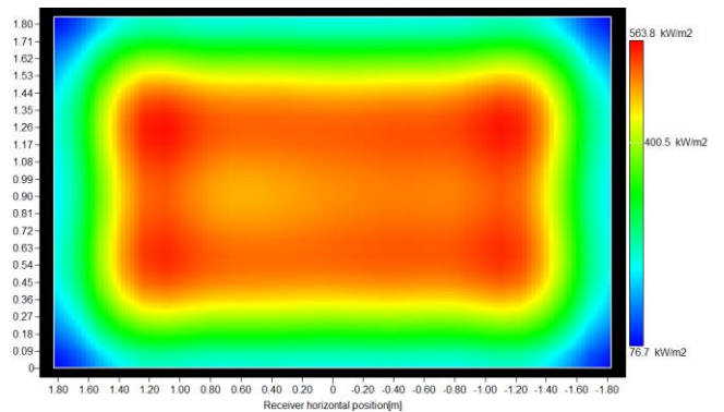
Figure 8. Incident flux on the receiver for SM 1.3 and heliostat type 3
