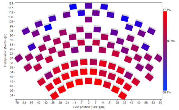
Figure 12. Solar field SM 1.2 Type 2 heliostats
