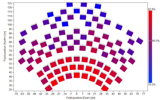
Figure 13. Solar field SM 1.3 Type 2 heliostats
