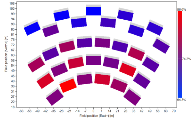
Figure 18. Solar field SM 1 Type 1 heliostats
