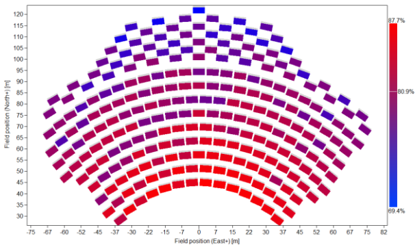
Figure 4. Solar field SM 1.3 Type 3 heliostats
