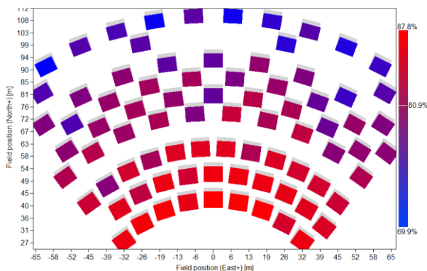
Figure 11. Solar field SM 1.1 Type 2 heliostats
