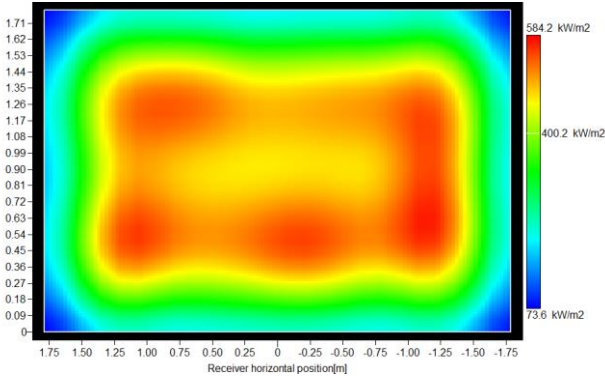
Figure 16. Incident flux on the receiver for SM 1.2 and heliostat type 2
