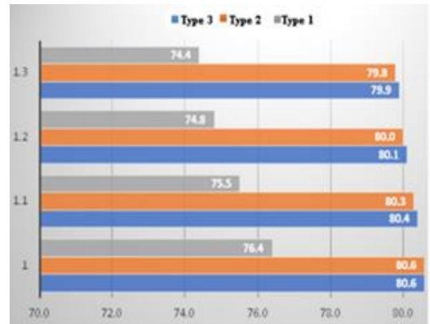
Figure 27. Solar field efficiency for the three heliostat sizes
