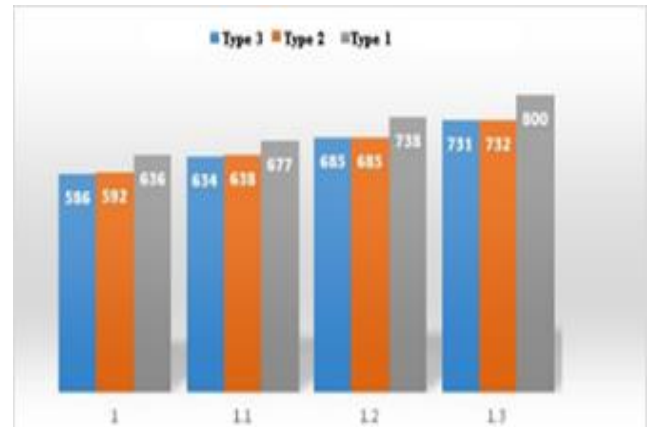
Figure 26. Concentration ratio for the three different kind of heliostats
