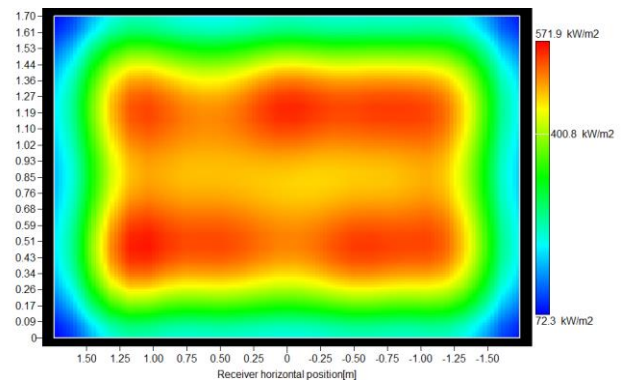
Figure 15. Incident flux on the receiver for SM 1.1 and heliostat type 2
