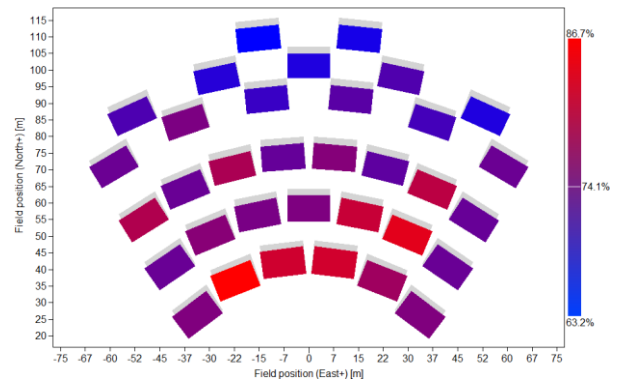
Figure 19. Solar field SM 1.1 Type 1 heliostats
