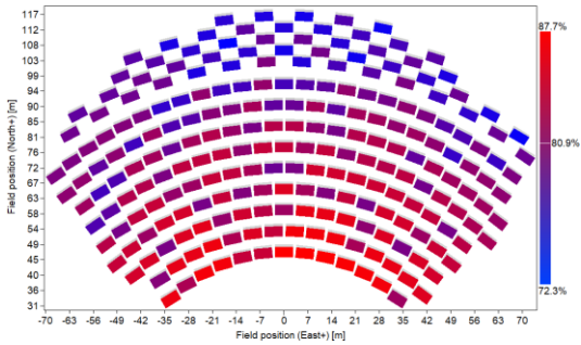
Figure 3. Solar field SM 1.2 Type 3 heliostats
