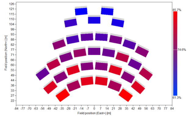
Figure 20. Solar field SM 1.2 Type 1 heliostats
