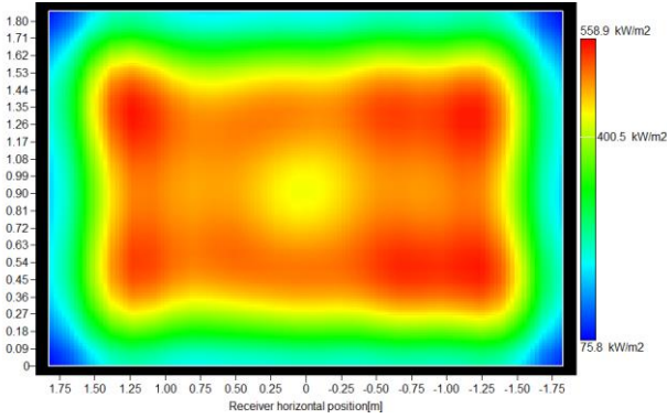
Figure 17. Incident flux on the receiver for SM 1.3 and heliostat type 2
