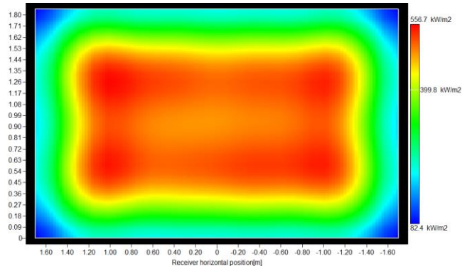
Figure 7. Incident flux on the receiver for SM 1.2 and heliostat type 3
