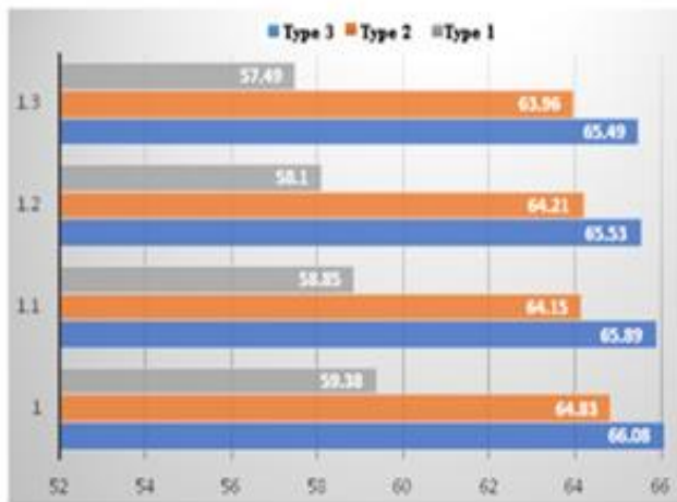
Figure 29. Annual efficiency for all configuration
