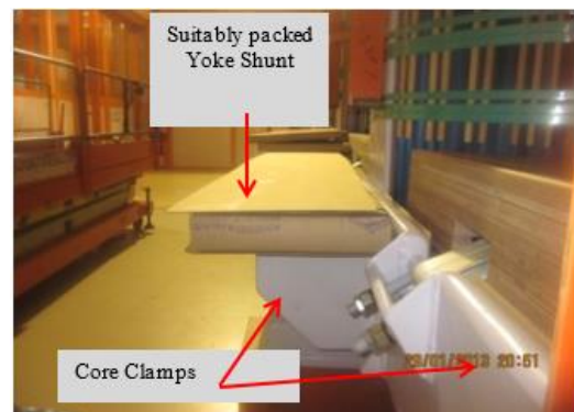
Figure 3. Location and arrangement of Yoke shunt
