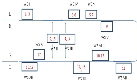
Figure 8. Sharing of tasks 15 & 14 by Workstations 2 & 3 for the Optimal Solution obtained By SAA for P19 [CT=6]
