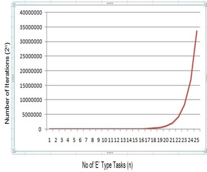
Figure 3. Number of Iteration of EHA Vs No of 'E' Type Tasks
