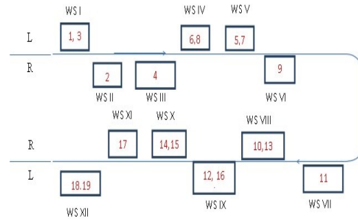
Figure 7. Allocation of tasks for the Optimal Solution obtained by SAA for P19
