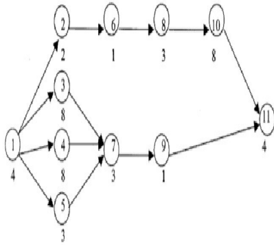
Figure 1. Precedence diagram and the task times of the example problem
