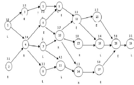
Figure 5. Precedence Diagram along with Task Time and Operation Directions of P19 – UALBP
