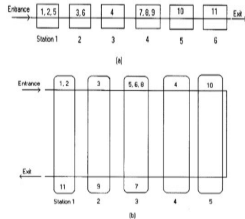
Figure 2. Schematic view of (a) straight line and (b) U-line configurations for the example problem.
