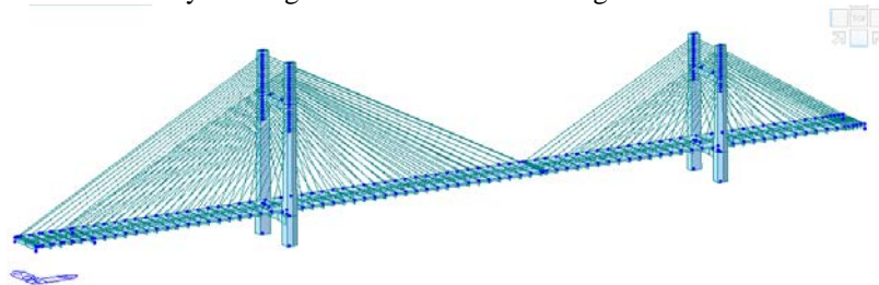
Figure.1 Finite element of full bridge
