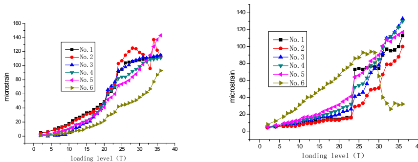
(a) The east cable concrete micro-strain change curve (b) The west cable concrete micro-strain change curve
