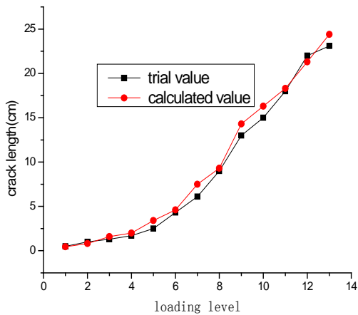
Figure.7 Crack length comparison of experimental and calculated value
