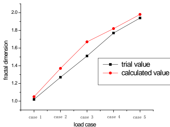
Figure.9 Compared with the finite element calculation results test
