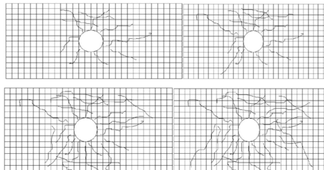
Figure.3 Crack distribution and mesh generation
