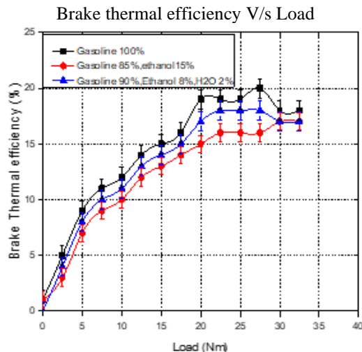
Figure 7. Plot between Brakethermal efficiency and Load
