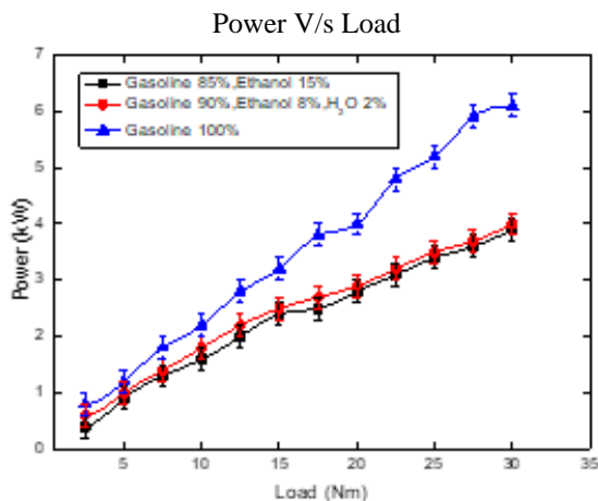
Figure 3. Plot between power and load
