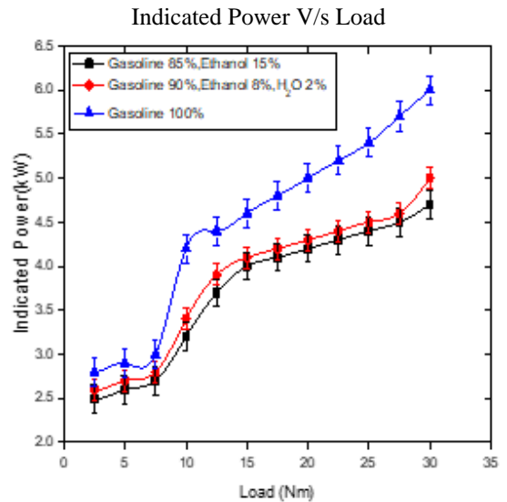
Figure 4. Plot between IP and load
