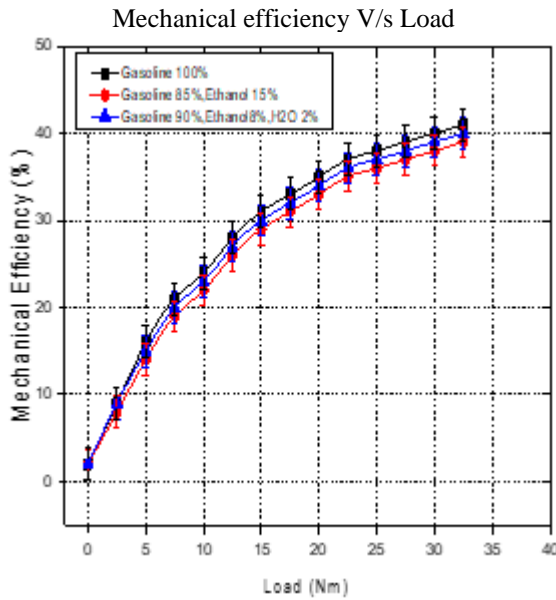
Figure 9. Plot between Mechanical efficiency and Load
