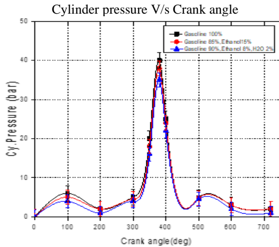
Figure 6. Plot between Cy. pressure and crank angle
