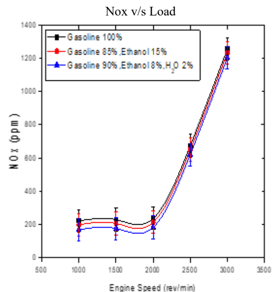
Figure 12. Plot between Nox and Engine Speed
