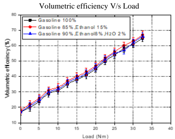
Figure 8. Plot between Volumetric efficiency and Load
