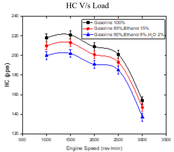
Figure 11. Plot between HC emissions and Engine Speed
