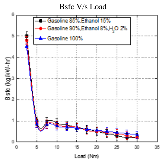
Figure 5. Plot between Bsfc and Load
