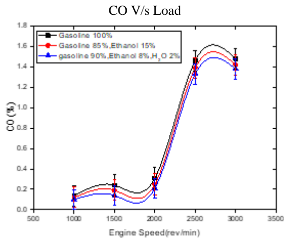
Figure 10. Plot between CO emissions and Engine Speed
