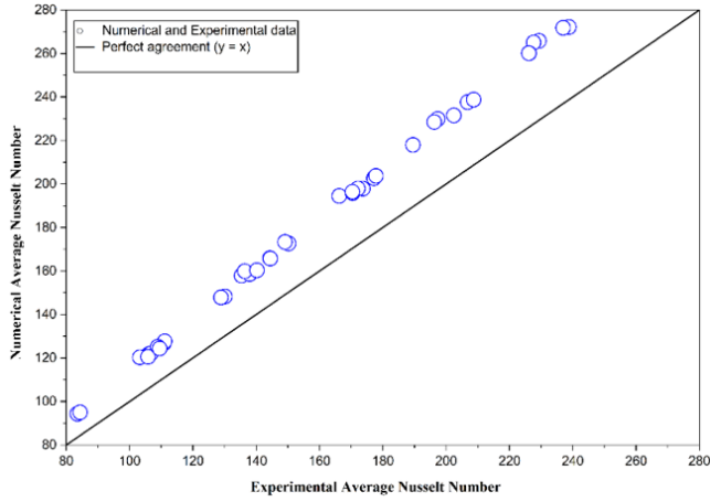
Figure 6. A comparison between the averaged Nusselt numbers ( Nu ) is shown comparing the experimental and numerically obtained values for all geometries and operating conditions over the considered Reynolds number ( Re ) range
