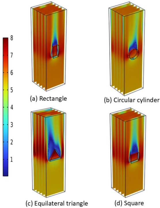
Figure 8. Velocity contours of the investigated geometries: (a) rectangle, (b) circular cylinder, (c) equilateral triangle, and (d) square at a heating power of 300 W and an air velocity of 6 m/s
