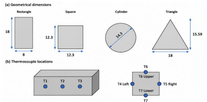
Figure 4. Dimensions of the investigated geometries and thermocouple locations
