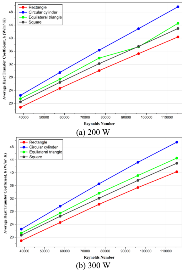
Figure 11. Variation of the average heat transfer coefficient (HTC) with Reynolds number ( Re ) for the investigated geometries at (a) 200 W and (b) 300 W
