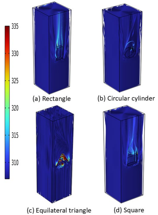
Figure 9. Temperature-colored streamlines for the investigated geometries, (a) rectangle, (b) circular cylinder, (c) equilateral triangle, and (d) square at a heating power of 300 W and an air velocity of 6 m/s
