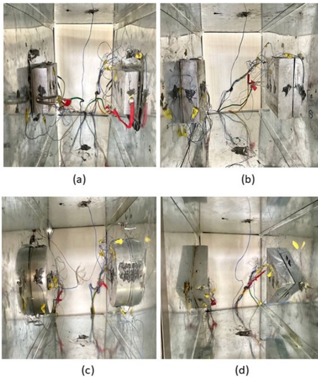
Figure 3. Photographs of the investigated obstacle configurations installed symmetrically inside the test section, (a) rectangle, (b) square, (c) circular cylinder, and (d) equilateral triangle obstacles
