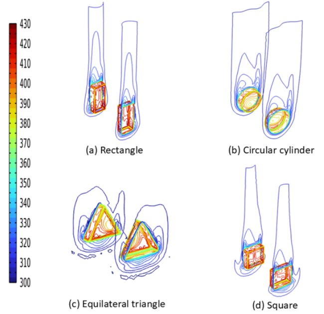
Figure 7. Temperature contours for the investigated geometries, (a) rectangle, (b) circular cylinder, (c) equilateral triangle, and (d) square at a heating power of 300 W and an air velocity of 6 m/s
