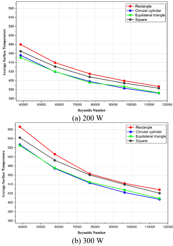
Figure 10. Variation of the average surface temperature with Reynolds number ( Re ) for the investigated geometries at (a) 200 W and (b) 300 W
