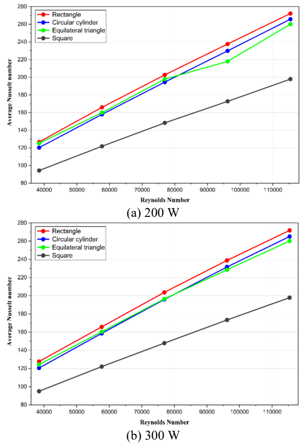
Figure 12. Variation of the average Nusselt number ( Nu ) with Reynolds number ( Re ) for the investigated geometries at (a) 200 W and (b) 300 W
