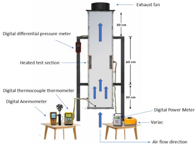
Figure 2. Schematic representation of the experimental setup showing the test airflow direction and measuring instruments
