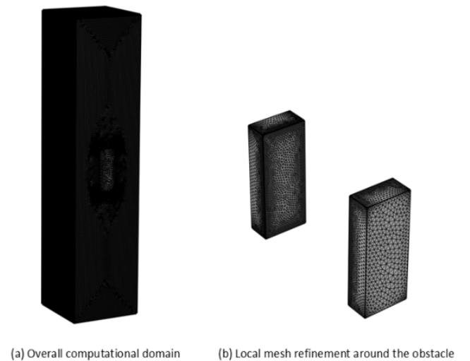
Figure 5. Computational mesh used in the numerical simulations, (a) overall computational domain and (b) local mesh refinement around the heated obstacle
