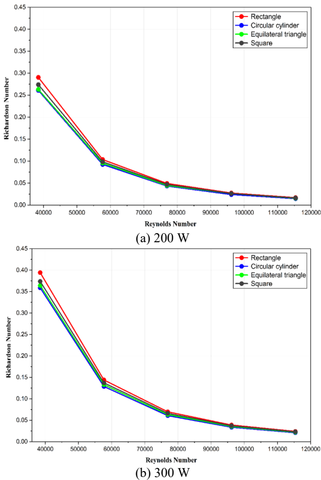
Figure 13. Variation of Richardson number ( Ri ) with Reynolds number ( Re ) for the investigated geometries at (a) 200 W and (b) 300 W
