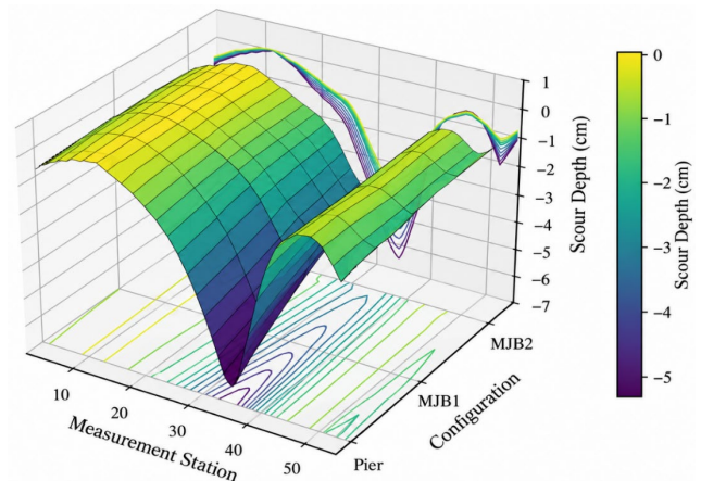
Figure 5. Longitudinal scour-depth profiles (cm) for the unprotected pier, MJB1, and MJB2 under Q_2
