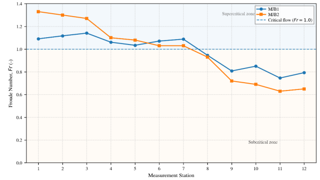
Figure 4. Longitudinal distribution of the Froude number ( Fr ) at measurement stations S1-S12 for MJB1 and MJB2 under Q_2
