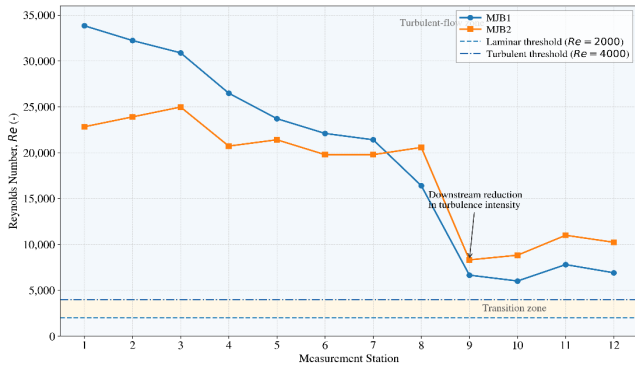
Figure 3. Longitudinal distribution of the depth-based Reynolds number ( Re ) at measurement stations S1-S12 for MJB1 and MJB2 under Q_2
