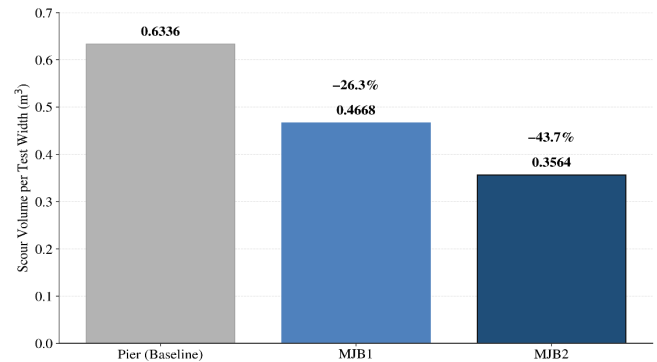
Figure 7. Total scour volume for the unprotected pier, MJB1, and MJB2 under Q_2
