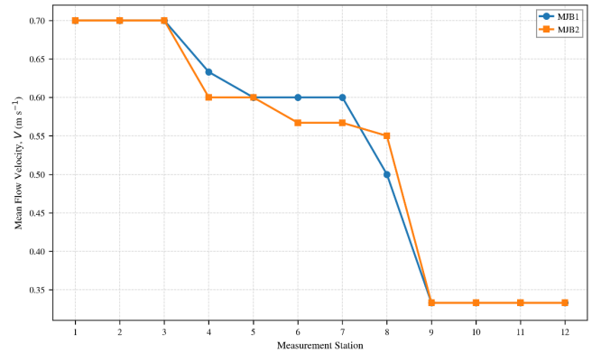
Figure 2. Longitudinal distribution of mean flow velocity ( m/s ) at measurement stations S1–S12 for the MJB1 and MJB2 porous-net configurations under the higher tested discharge condition ( Q_2 )
