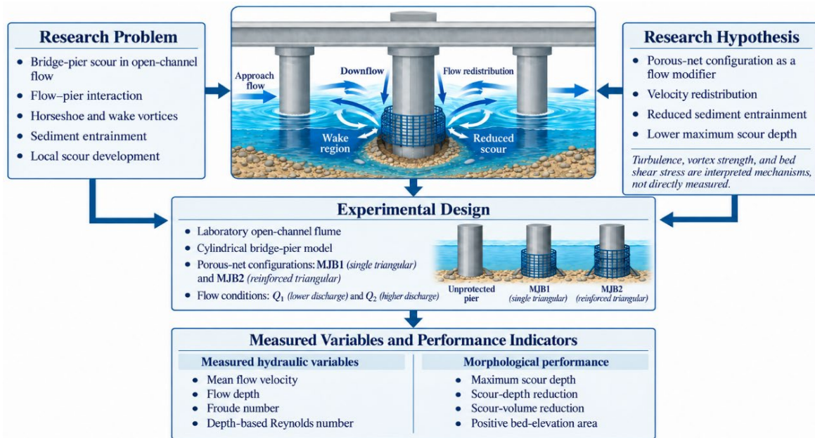
Figure 1. Conceptual framework of hydrodynamic scour mitigation using porous net structures
