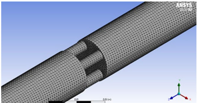
Figure 5. Magnifier photo for mesh of one plate
