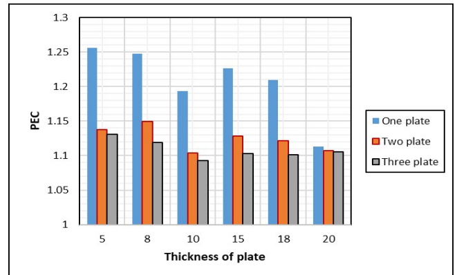
Figure 17. Performance evaluation criteria (PEC) for circular holes at different numbers of plates at Re = 1500
