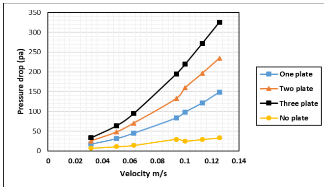
Figure 13. Pressure drop versus velocity for circular holes and a thickness of 5 mm at different numbers of plates
