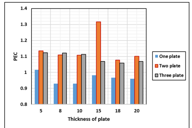
Figure 18. Performance evaluation criteria (PEC) for rectangular holes for different numbers of plates at Re = 1500
