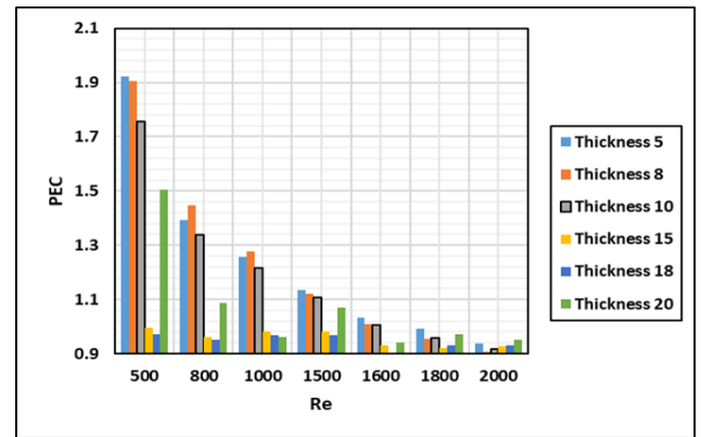
Figure 16. Performance evaluation criteria (PEC) for rectangular holes for different thicknesses for two plates
