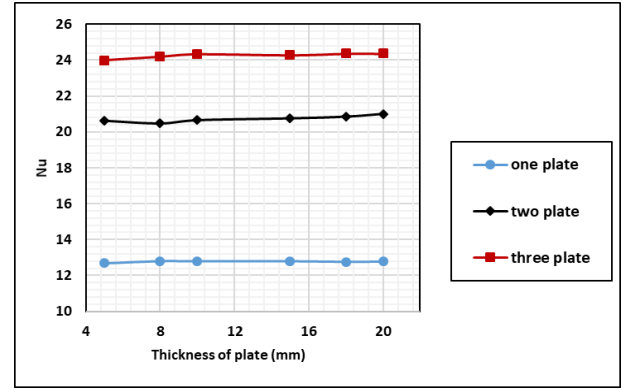
Figure 10. Nu versus thickness of plates for rectangular holes at Re = 1000
