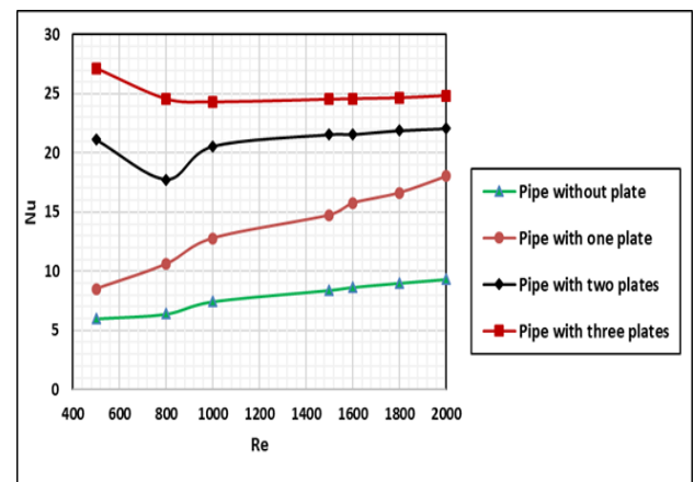
Figure 7. Nu versus Re at different numbers of plates with rectangular holes and a thickness of 10 mm
