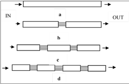
Figure 3. Geometry model: a- pipe without plate b-pipe with one plate c- pipe with two plates d- pipe with three plates
