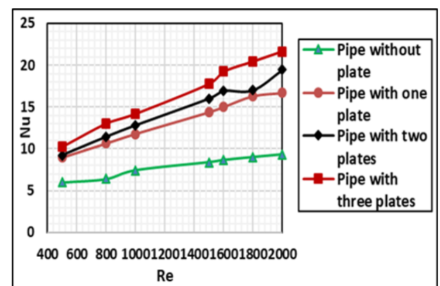
Figure 8. Nu versus Re at different numbers of plates with circular holes and a thickness of 10 mm
