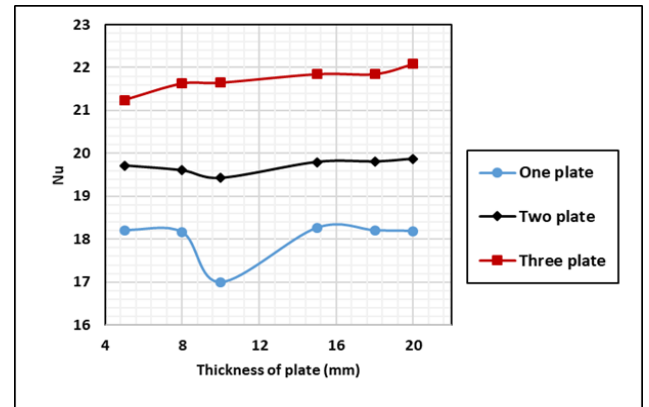
Figure 11. Nu versus thickness of plates for circular holes at Re = 1000
