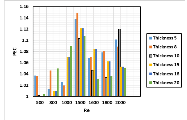
Figure 15. Performance evaluation criteria (PEC) for circular holes for different thicknesses for two plates
