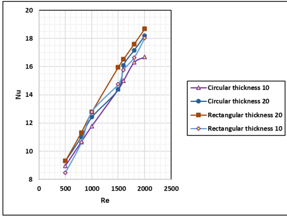
Figure 12. Nu versus Re for two shape holes for one plate and different thicknesses
