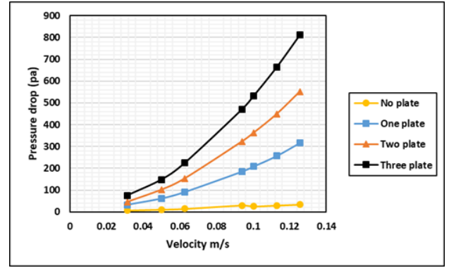
Figure 14. Pressure drop versus velocity for rectangular holes and a thickness of 5 mm at different numbers of plates
