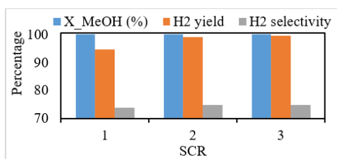
Figure 6. Effect of varying steam-to-methanol ratio (SCR) on methanol conversion, hydrogen yield and hydrogen selectivity
