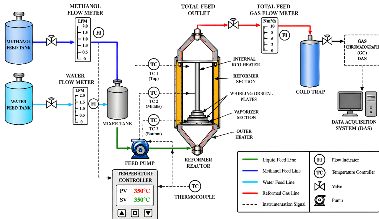
Figure 1. Process flow diagram of the Methanol Steam Reforming (MSR) process
