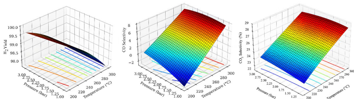
Figure 8. Effect of temperature and pressure on (a) hydrogen yield, (b) CO selectivity, (c) CO 2 selectivity
