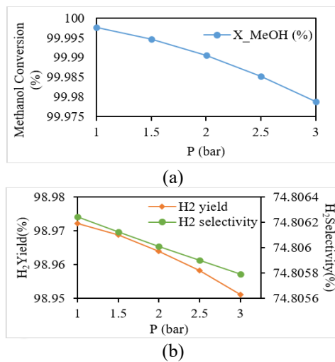
Figure 5. Effect of varying pressure on (a) methanol conversion, (b) hydrogen yield and hydrogen selectivity
