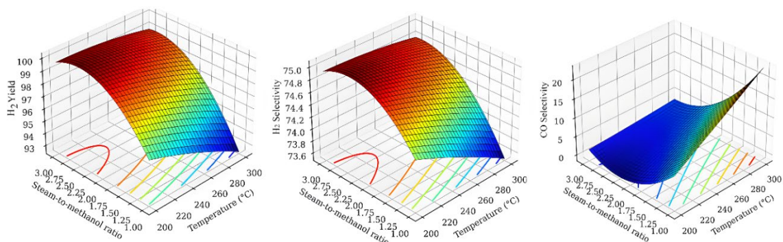
Figure 7. Effect of temperature and steam-to-methanol ratio (SCR) on (a) hydrogen yield, (b) hydrogen selectivity, (c) CO selectivity
