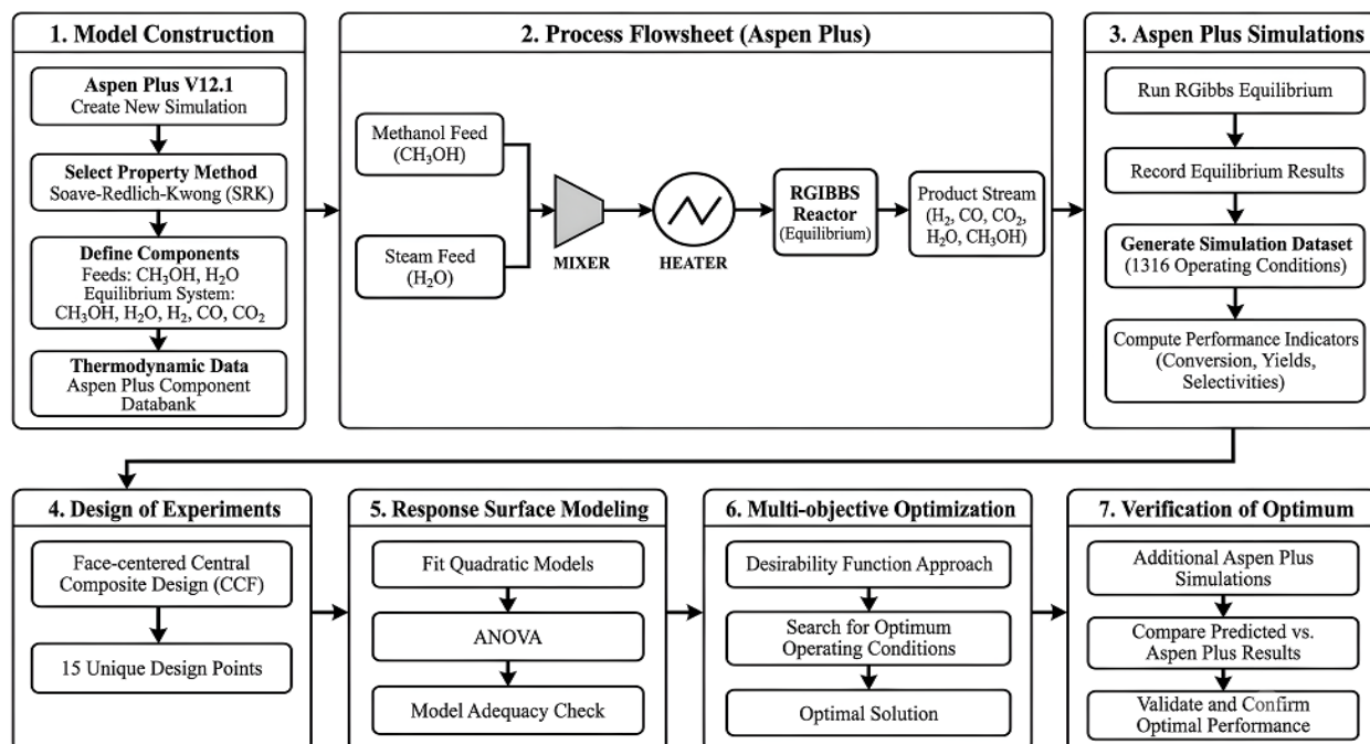
Figure 3. Flow diagram of workflow with Aspen Plus-RGibbs response surface methodology (RSM) optimization
