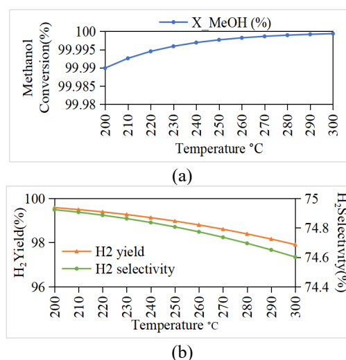
Figure 4. Effect of varying temperature on (a) methanol conversion, (b) hydrogen yield and hydrogen selectivity
