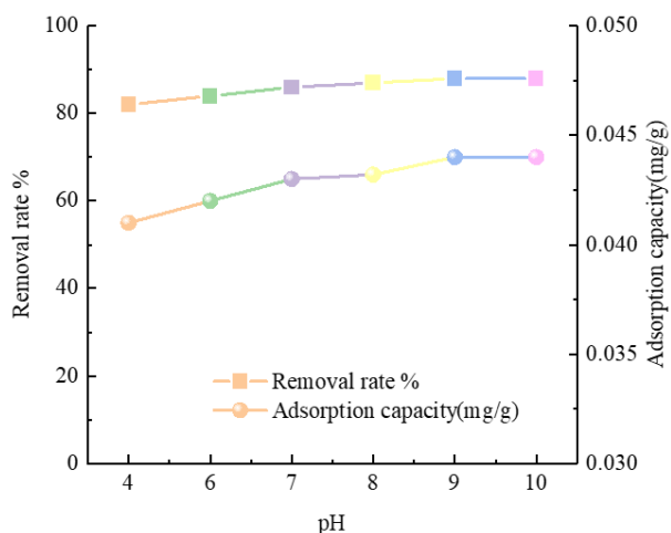
(a) Effect of raw water pH on adsorption performance
