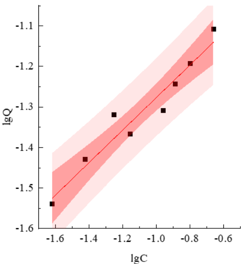
(b) Freundlich adsorption isotherm fitting plot
