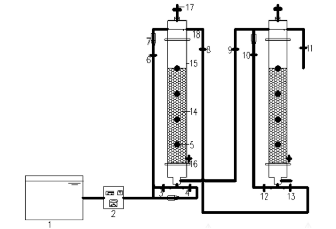
Figure 1. Schematic diagram of the dynamic adsorption experimental setup Note: 1. Water tank 2. Peristaltic pump 3. Valve 4. Valve 5. Water sampling port 6, 8–13 Valves 7. Flowmeter 14. Modified zeolite 15. Fixed adsorption column 16. Support layer 17. Exhaust port 18. Pipe connection.
