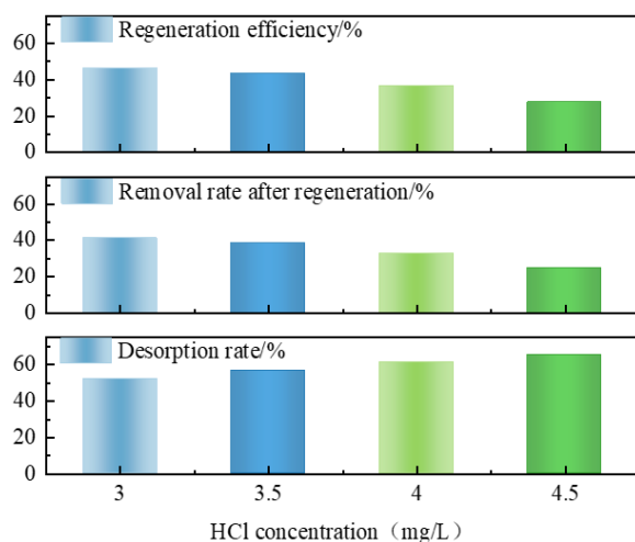
(c) Effect of HCl concentration on regeneration performance
