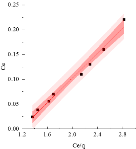
(a) Langmuir adsorption isotherm fitting plot
