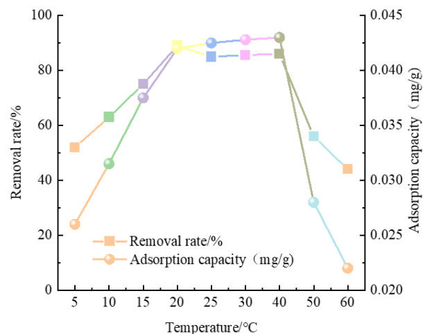
(f) Effect of reaction temperature on adsorption performance
