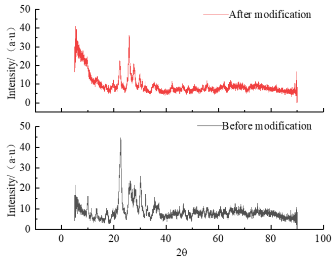
Figure 3. X-ray Diffraction (XRD) pattern analysis
