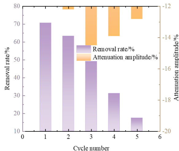
(d) Removal rate and attenuation trend over five adsorption-regeneration cycles
