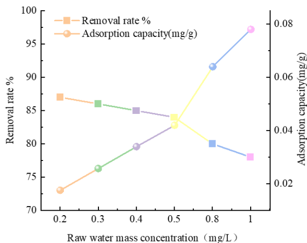
(c) Effect of raw water mass concentration on adsorption performance
