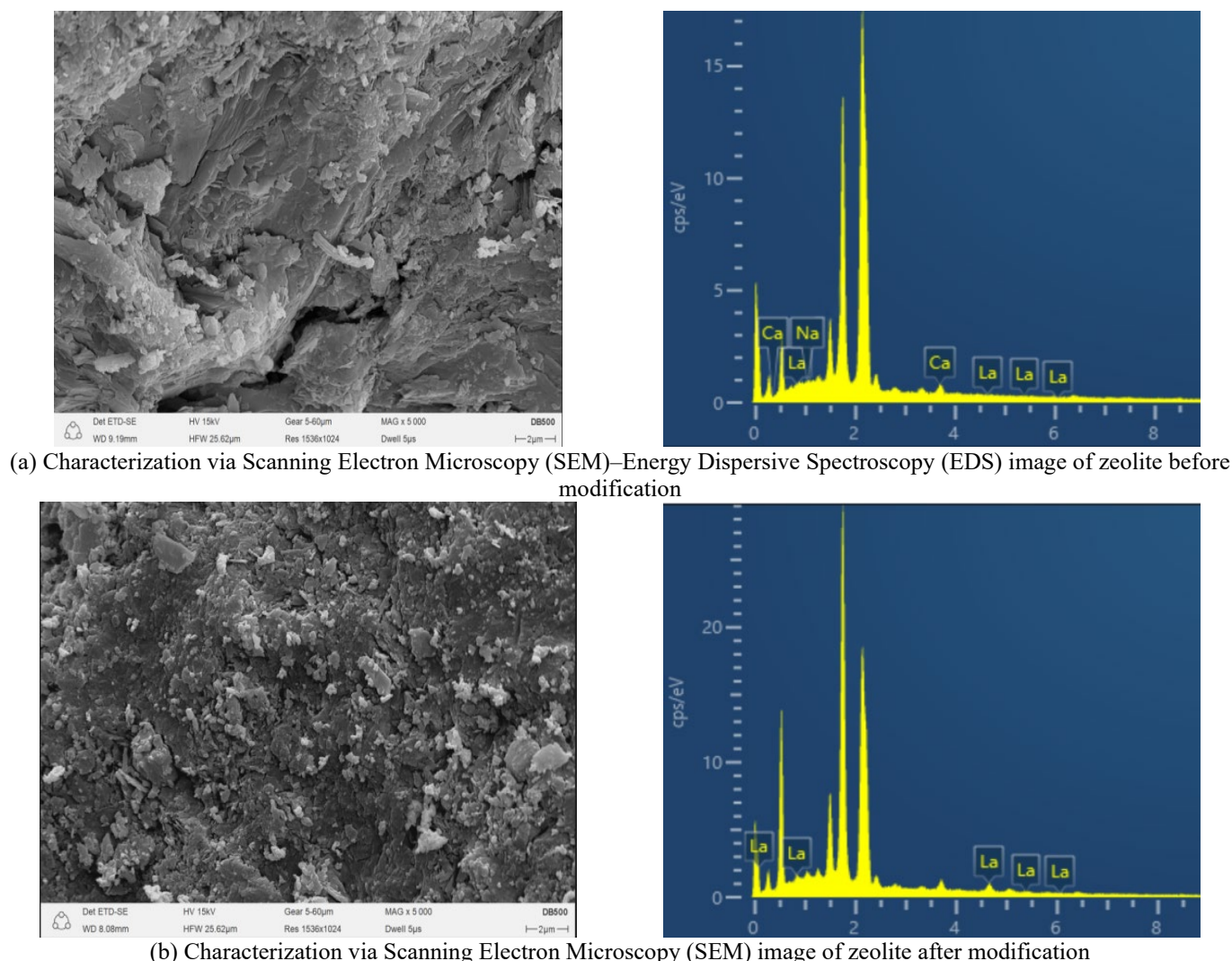
Figure 2. Characterization via Scanning Electron Microscopy (SEM)–Energy Dispersive Spectroscopy (EDS) analysis results
