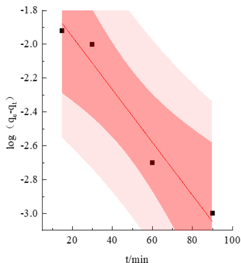
(c) Pseudo-first-order kinetics fitting trend line
