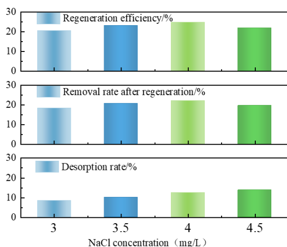
(a) Effect of NaCl concentration on regeneration performance
