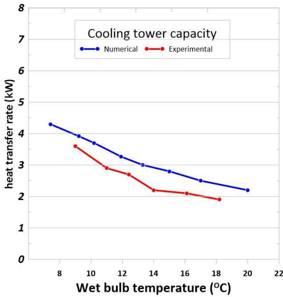
Figure 12. The validation between numerical and experimental heat transfer rate
