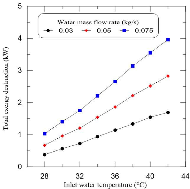
Figure 9. Total exergy destruction
