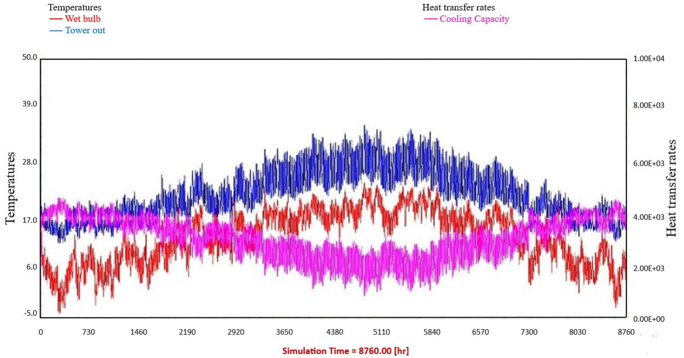
Figure 11. Variation of the outlet water temperature, wet bulb ambient temperature, and cooling capacity
