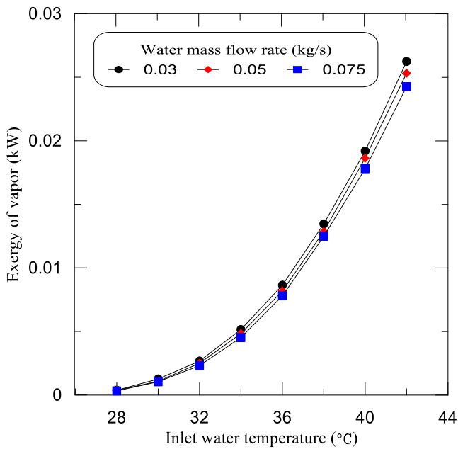
Figure 8. Exergy of the vapor
