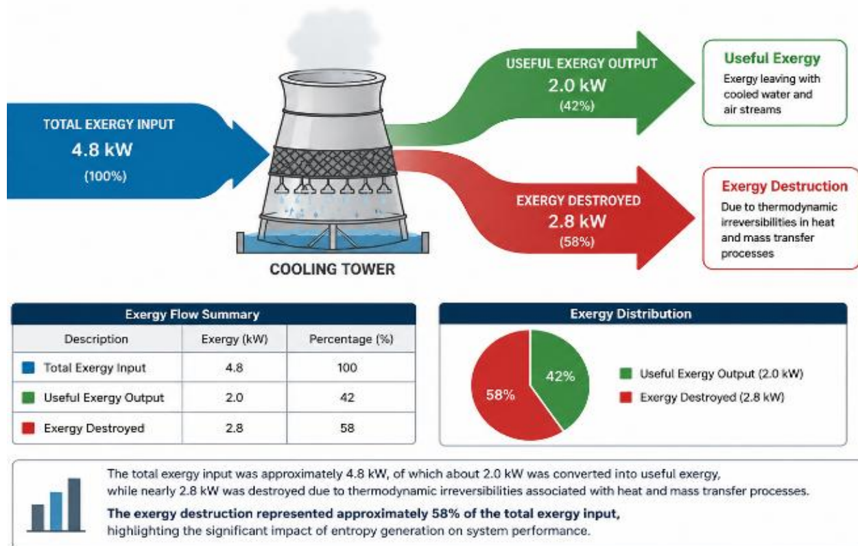
Figure 13. The exergy flow distribution through the cooling tower
