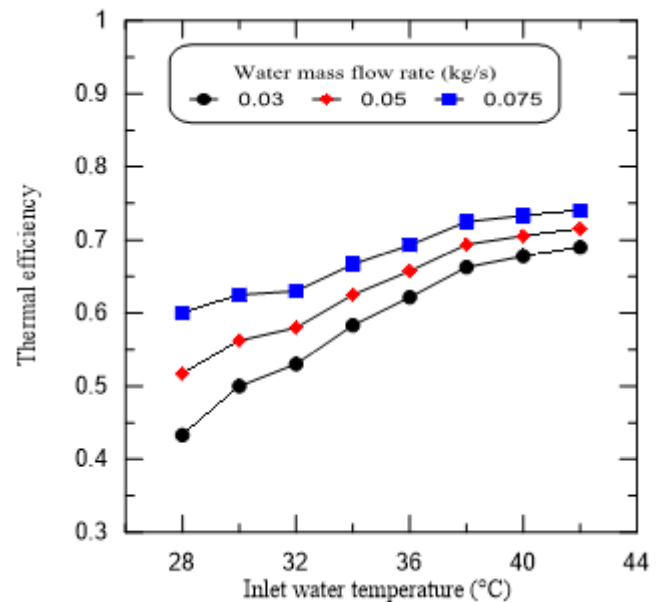
Figure 4. Thermal efficiency of the cooling tower
