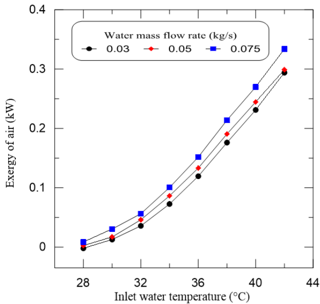
Figure 6. The exergy of humid air
