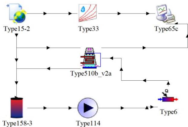
Figure 3. The schematic diagram of the developed model in TRNSYS simulation studio
