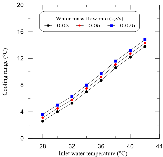
Figure 5. The cooling tower range
