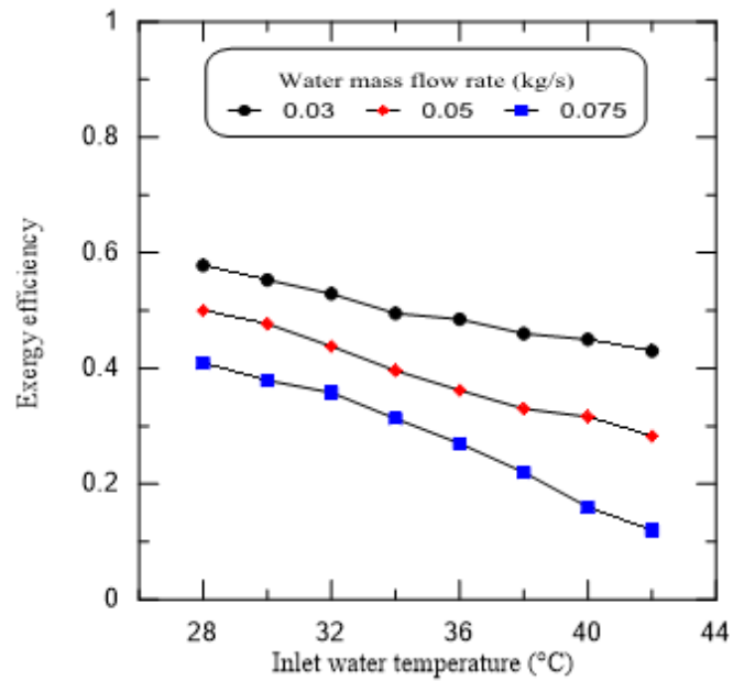
Figure 10. The cooling tower exergy efficiency
