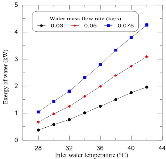
Figure 7. The exergy of water
