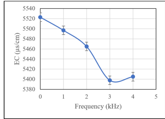
Figure 12. Electric conductivity vs. frequency of square wave for salt water
