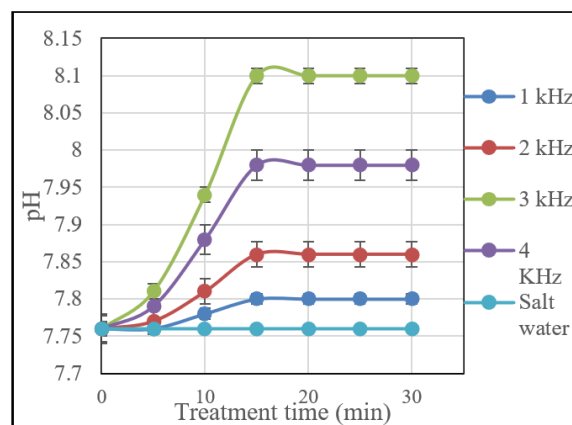
Figure 9. pH vs. treatment time for salt water
