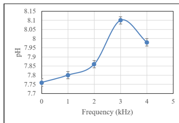
Figure 10. pH vs. frequency of the square wave for salt water
