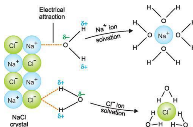
Figure 1. \text{Na}^+ and \text{Cl}^- ions hydration [1]
