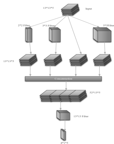
Figure 3. A convolutional neural network (CNN) model for image enhancement
