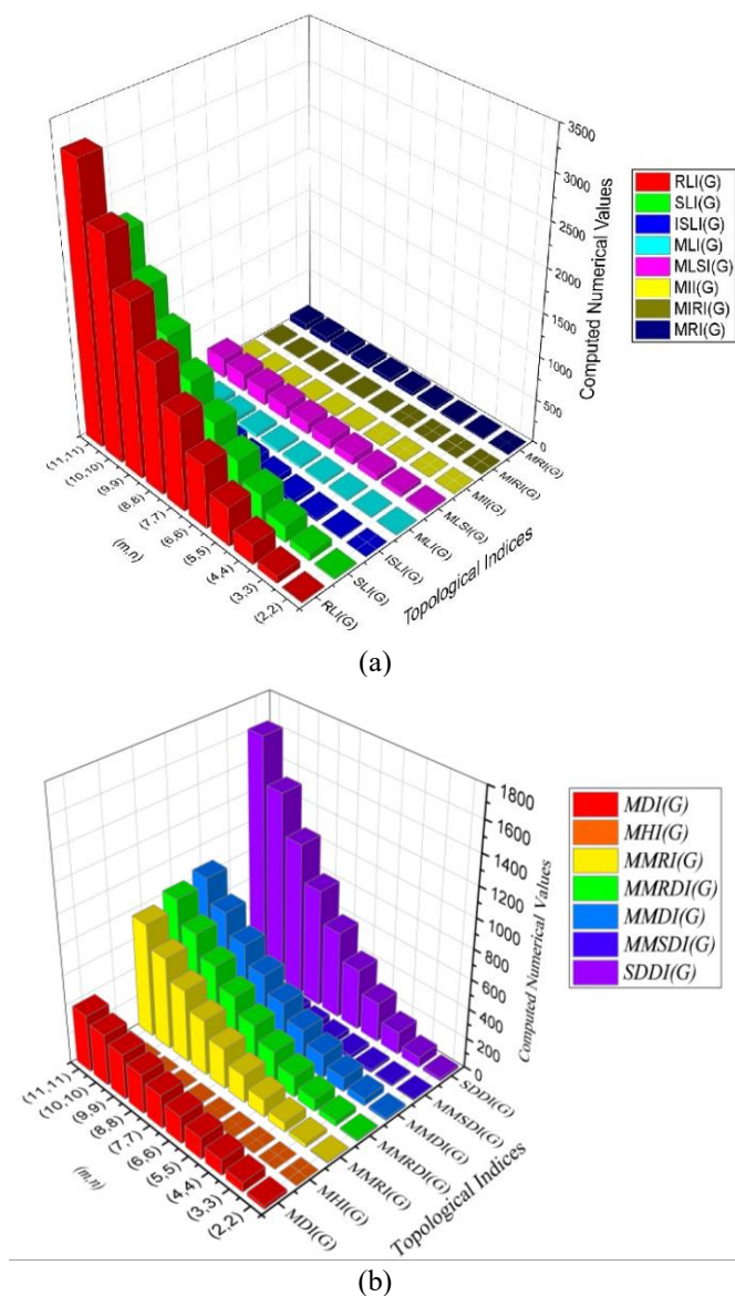
Figure 8. A visual representation of molecular characteristics for bond addition of mesh derived network MDN_2(m, n)
