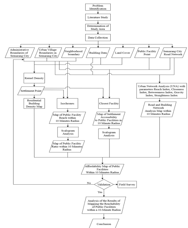
Figure 1. Methodological framework
