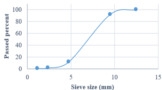
Figure 1. Grading of the utilized gravel
