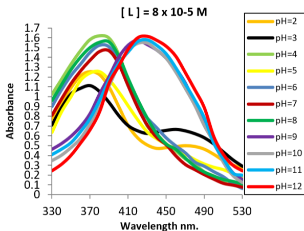
Figure 5. The electronic spectra of azo dye L at different pH values
