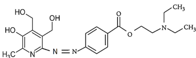
Scheme 1. Azo dye L. L: 2-(diethylamino) ethyl Z-4-[(5-hydroxyl-3,4-bis(hydroxymethyl)-6-methylpyridin-2-yl] benzoate
