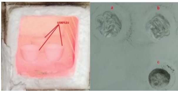
Figure 3. Calcination process with in a muffle furnace is carried out at 1000°C for a) 20%LHA b) 40%LHA c) 60%LHA
