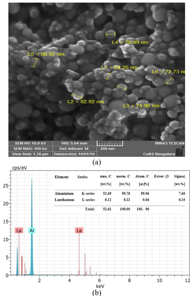
Figure 7. (a) FESEM Grain size measurement and EDX report for 20 vol% LHA sample calcinated at 1000°C, (b) EDX report for 20 vol% LHA sample calcinated at 1000°C
