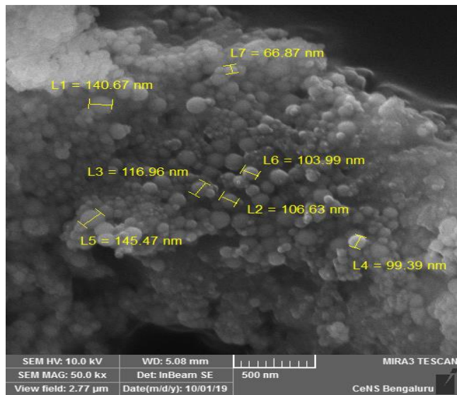
Figure 8. (a) FESEM Grain size measurement and EDX report for 40 vol% LHA sample calcinated at 1000°C, (b) EDX report for 40 vol% LHA sample calcinated at 1000°C
