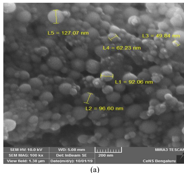
Figure 7. (a) FESEM Grain size measurement and EDX report for 20 vol% LHA sample calcinated at 1000°C, (b) EDX report for 20 vol% LHA sample calcinated at 1000°C
