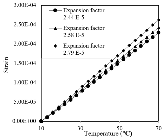
Figure 8. The relationship between temperature and strains for expansion factors
