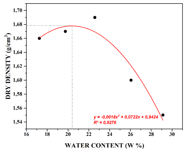
Figure 6. Compaction curve for Chott el Hodna clay
