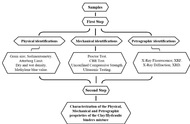
Figure 3. Flow chart of testing programme
