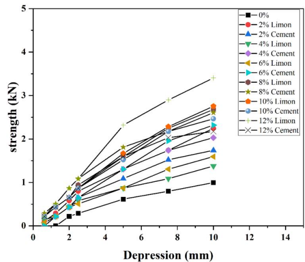
Figure 10. Effect of treatment on compressive strength
