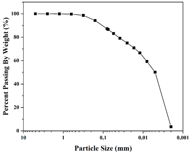
Figure 4. Grain size distribution curve of Chott el Hodna clay
