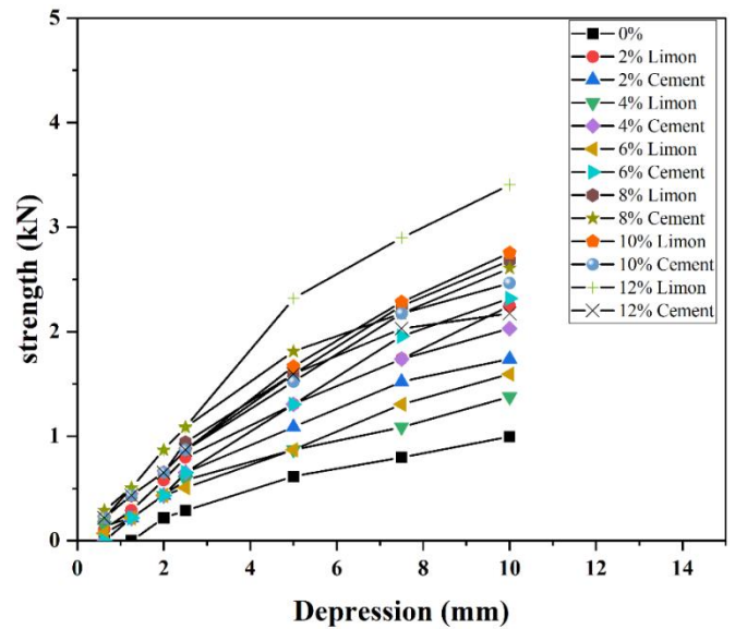
Figure 9. CBR Test results for clay and treatment mixtures
