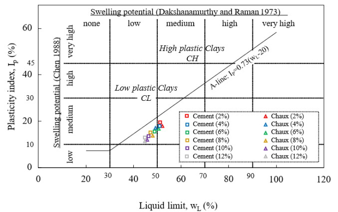
Figure 8. Treatment effect on the plasticity of the clay
