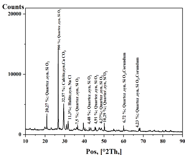
Figure 7. X-ray diffractogram of the studied clay
