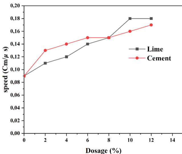
Figure 11. Speed of ultrasonic waves through soil samples treated with various dosages of lime and cement
