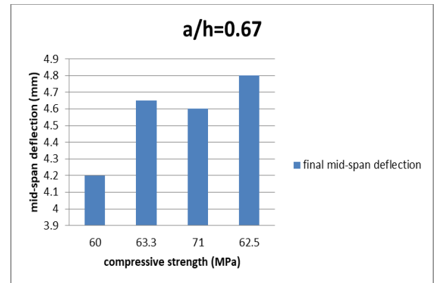
Figure 17. Effect compressive strength on mid-span deflection ( a/h=0.67 )
