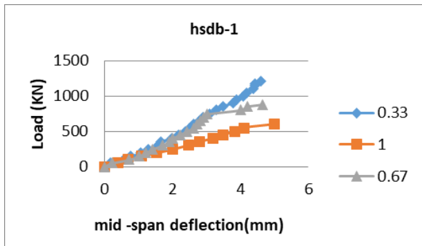
Figure 13. HSDB-1 specimens
