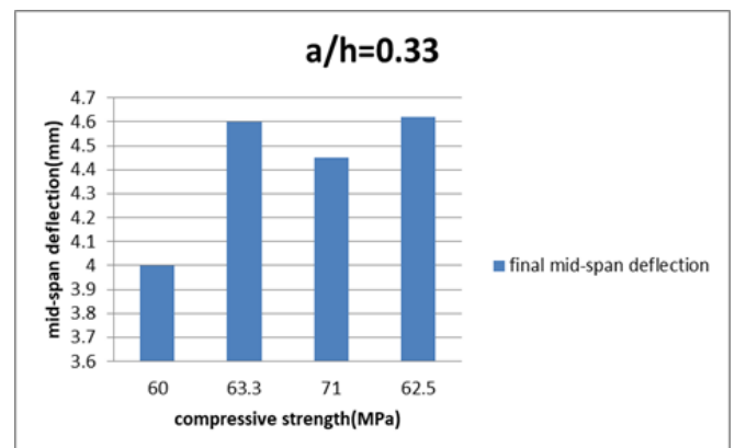
Figure 18. Effect compressive strength on mid-span deflection ( a/h=0.33 )
