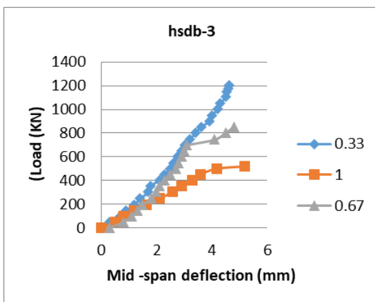
Figure 15. HSDB-3 specimens
