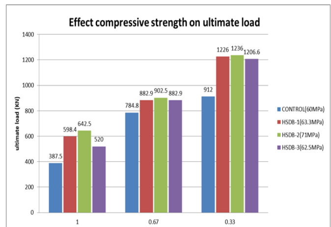
Figure 11. Effect compressive strength on the ultimate failure load
