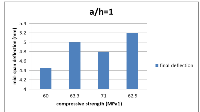
Figure 16. Effect compressive strength on mid-span deflection ( a/h=1 )
