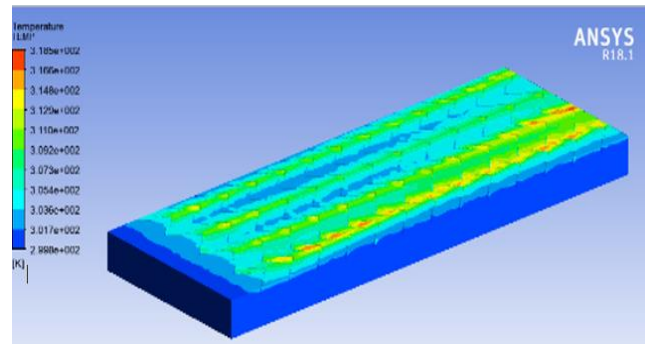
Figure 14. Temperature plot at 3900 Reynolds number
