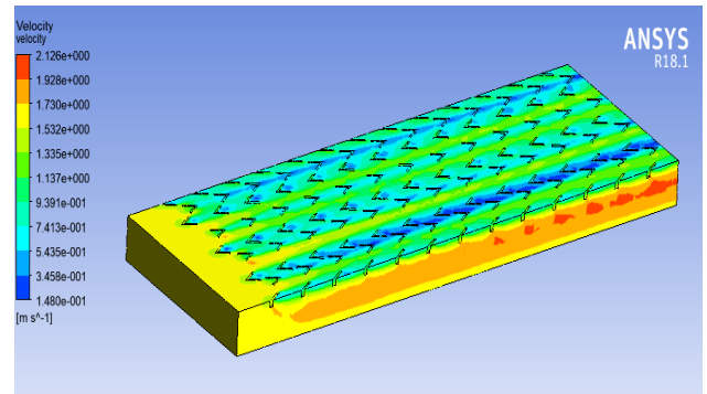
Figure 13. Velocity plot at 3900 Reynolds number
