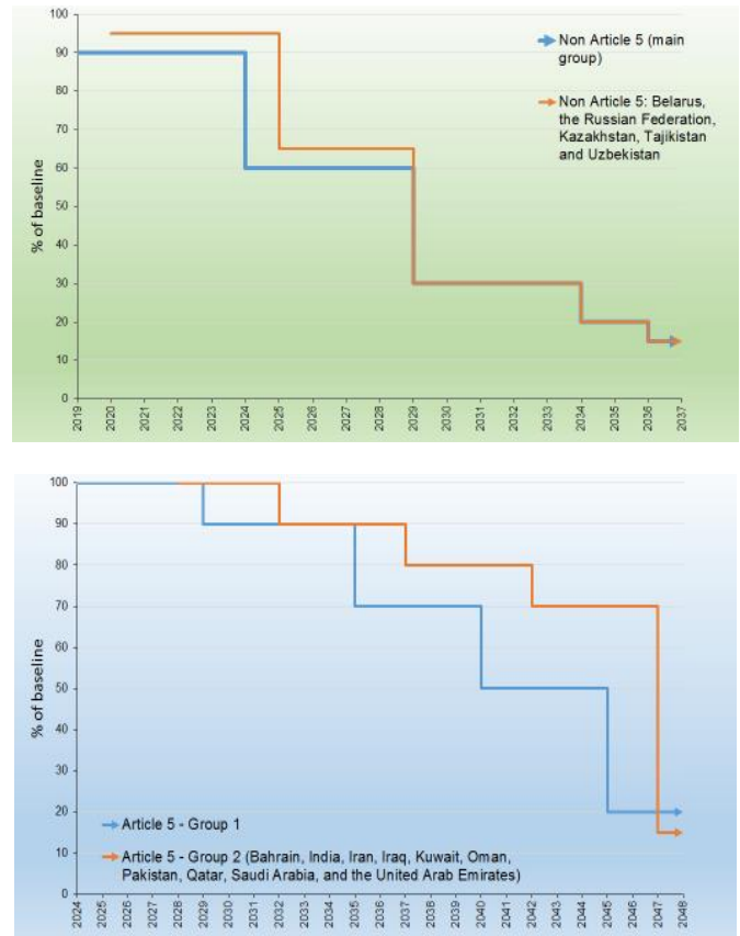
Figure 1. Kigali Amendment baseline calculation and phase-down schedules for non-A5 Parties (a) and A5 Parties (b) [6]
