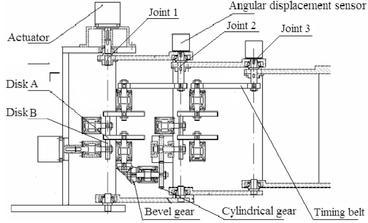
Fig. 3. Structural Diagram of Three Joints Nonholonomic Manipulator
