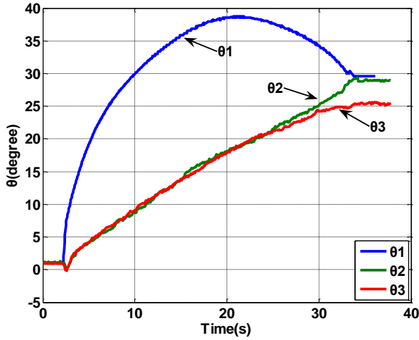
Fig.9. Joint Angles Displacement (Experiment)
