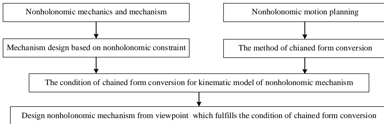
Fig. 1. Design of Controllable Nonholonomic Mechanical System
