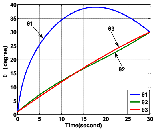
Fig.6. Joint Angles Displacement (Simulation)
