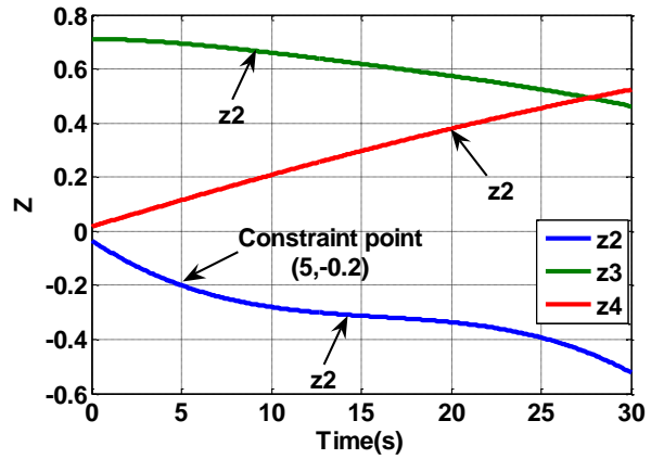
Fig.5. Control parameters z with one constraint point versus time
