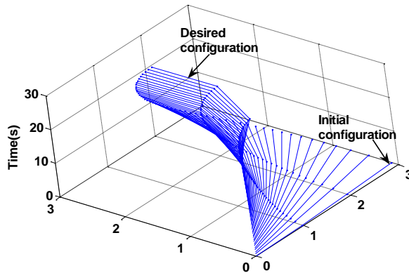
Fig.8. Three Nonholonomic Manipulator Motion in IR2
