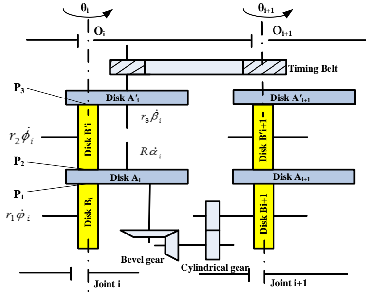
Fig.2. Structure Diagram of Joint i Mechanical System
