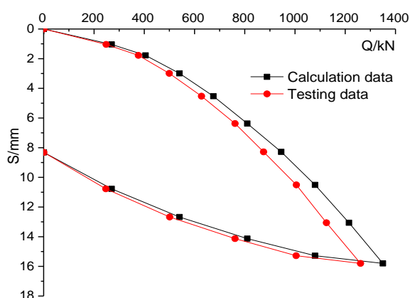
Fig.5. Comparison of Measured Value and Calculated Value (CFG Pile)
