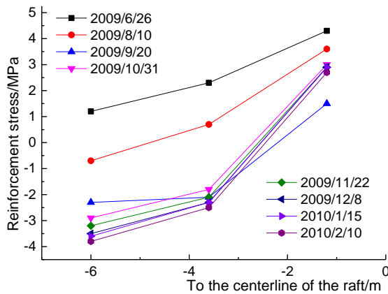
Fig.12. Vertical Reinforcement Distribution of the Rafts of PHC Pile-raft Composite Foundations
