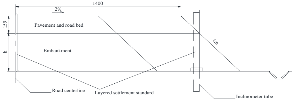
Fig.6. Deformation Monitoring Elevation Layout Drawing
