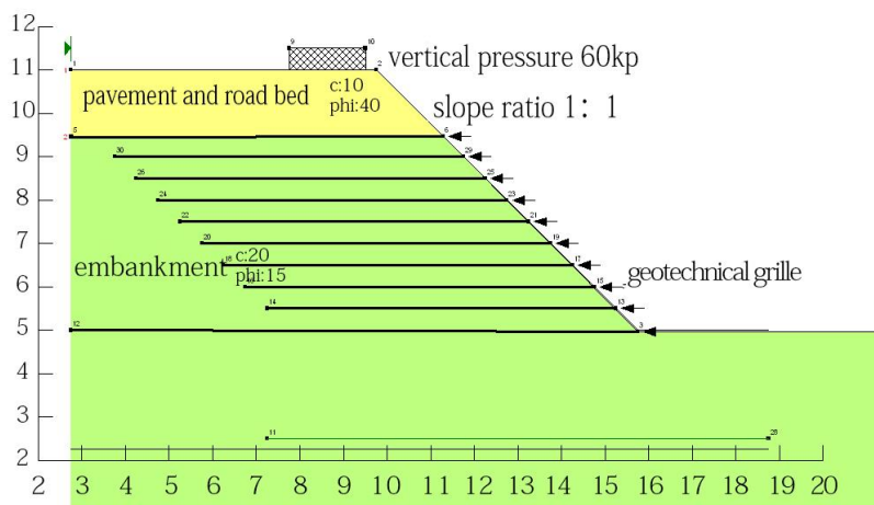
Fig.19. The Model of Geotechnical Grille Reinforced Embankment
