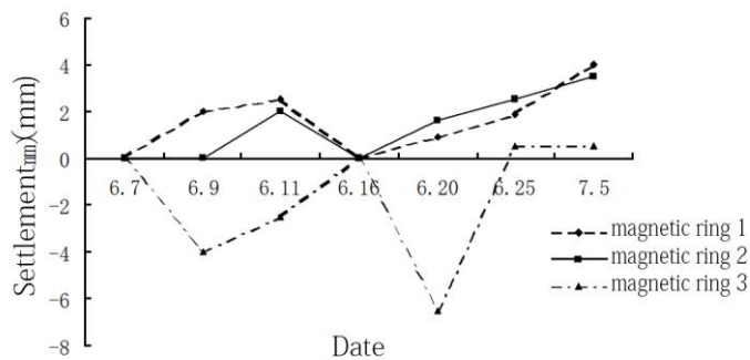
Fig.7. K243+900 Left Settlement
