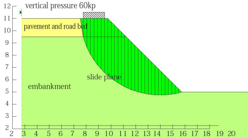
Fig.18. The Slide Plane Diagram of Steep Embankment (slope ratio 1:1)
