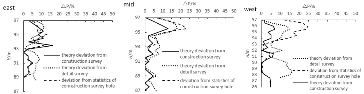
Fig.5. Rock embedding probability error curves of pile groups
