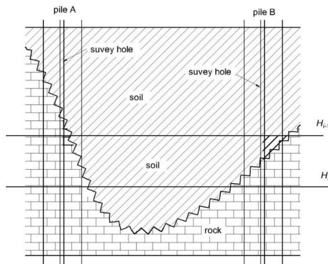
Fig. 1. rock-embedding relations between survey hole and pile
