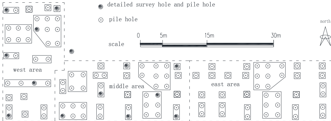
Fig.2. Floor plan for the pile foundation
