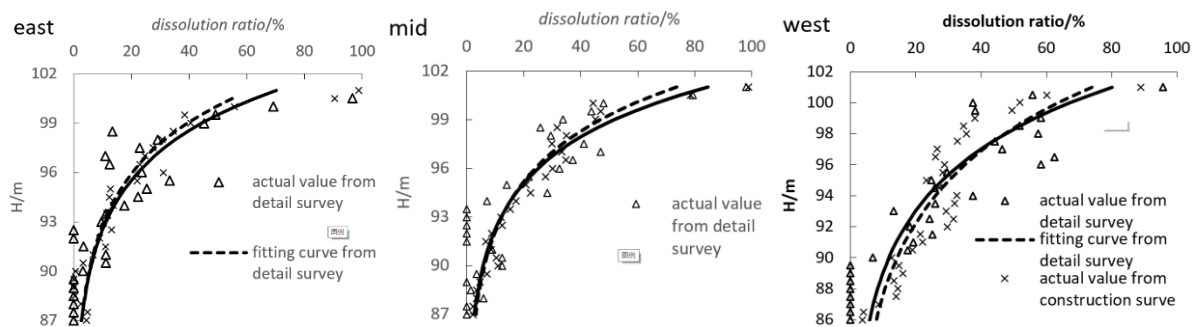
Fig.3. Depth distribution curve of the dissolution ratio
