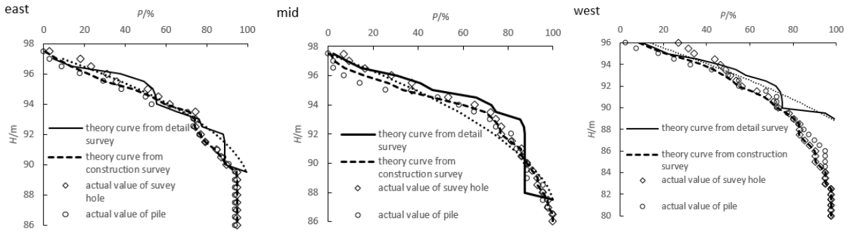
Fig.4. Rock embedding probability curves of pile groups
