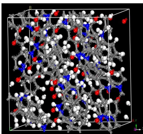
(a) PCFF force field
