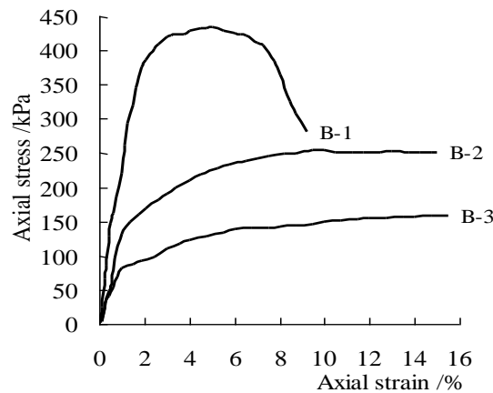
Fig.5. Stress-strain of Layered Mudstone Samples as a Function of Soft Interlayer Thickness Under Uniaxial Compression
