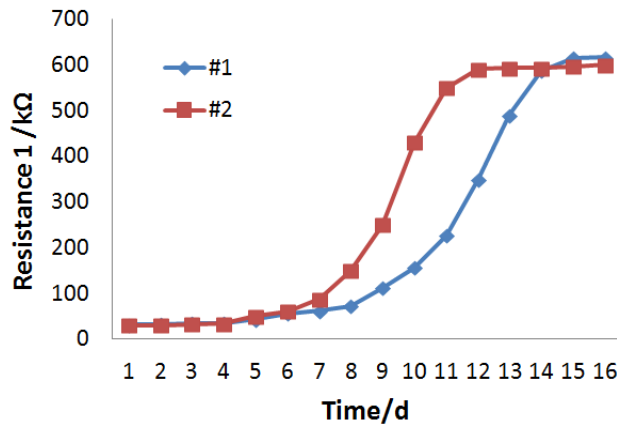
Fig.6. Variation Law of R1
