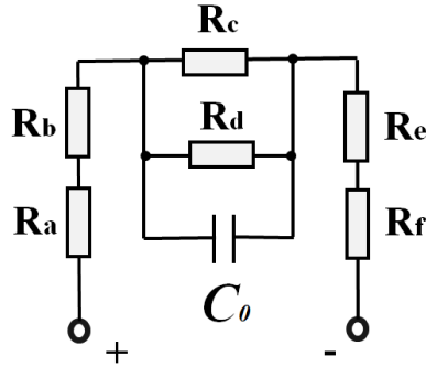
Fig.2. Electro-osmosis Equivalent Circuit Diagram
