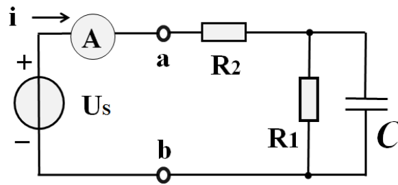
Fig.4. One Order RC Zero State Circuit
