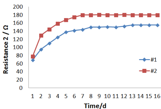
Fig.7. Variation Law of R_2
