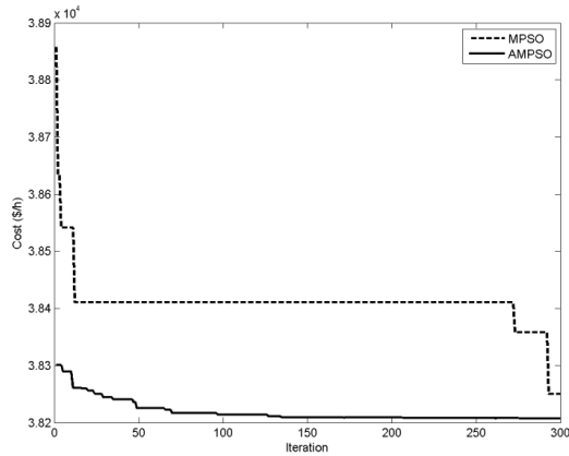
Figure 3. The lowest cost per iteration for a system of 6 generators with a demand of 700 megawatts
