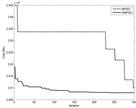
Figure 2. The lowest cost per iteration for a system of 6 generators with a demand of 500 megawatts
