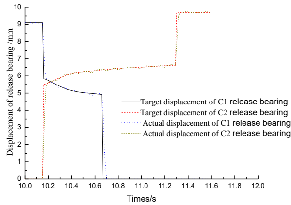
b. Displacement of release bearing
