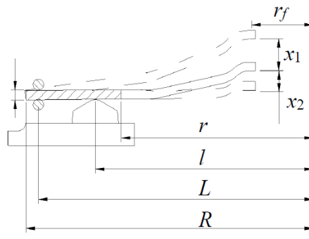
Fig.3. Schematic diagram of lever spring
