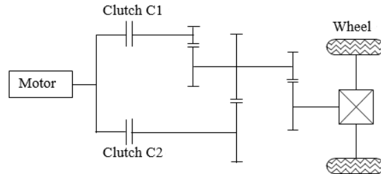
Fig.1. Working principle of electric vehicle
