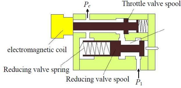
Fig.4. Principle diagram of proportional flow valve
