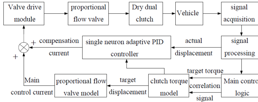
Fig.6. Control schematic diagram of dry dual clutch
