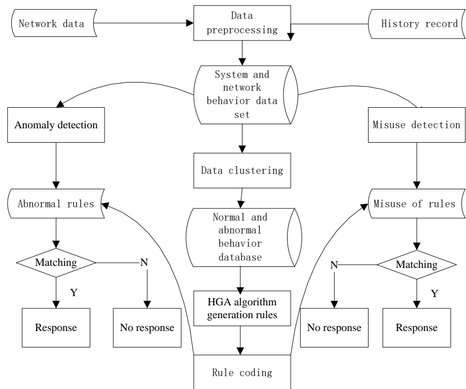
Fig.1. Structure of the Adaptive IDS Model
